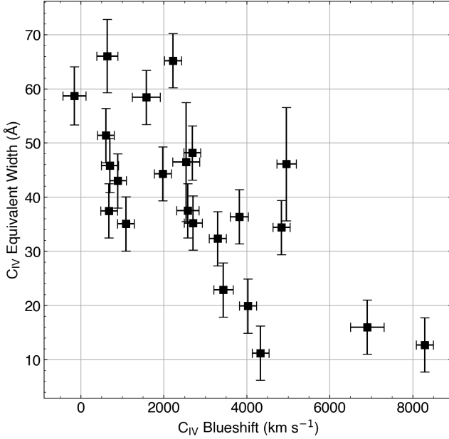
Figure 2. C IV equivalent width as a function of C IV blueshift. There is a moderate anti-correlation between these two quantities, implying that weaker C IV lines are more strongly blueshifted and stronger lines are less blueshifted. The outlier with high EW and blueshift is J1216+4519. Its SNR is low ( \sim 7 per pixel) which is reflected by the large error in EW.
