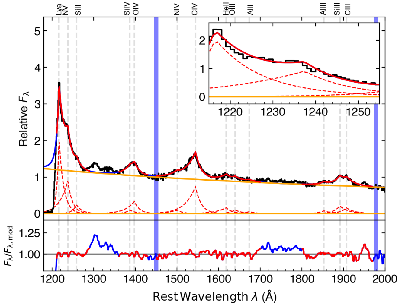
Figure 4. Example fit to ATLASJ029-36 observed using VLT/X-shooter with a mean SNR per 1\text{\AA} pixel of 27.35 between 1400\text{--}1600\text{\AA} . The top plot shows the spectrum after the post-processing techniques and the bottom plot shows the residuals. The inset plot provides a closer look at the line profiles of Ly \alpha and N v. The vertical blue bars indicate the continuum fitting windows, which are fit by the power-law continuum denoted by the orange line. The red lines indicate the emission line fits as well as the extent of the individual line-fitting windows. All fitted emission lines are labeled and their individual line profiles are shown.
