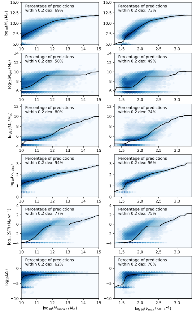
Figure B1. Relations between features commonly used in SHAM approaches (Subhalo mass and V_{\text{max}} ; x-axis) and each predictor (y-axis). Each panel shows a 2D histogram of the distribution (blue) alongside a fitted monotonic linear relation (black line). The percentage of galaxies where the predicted value is within 0.2 dex of the true value is quoted in each panel.
