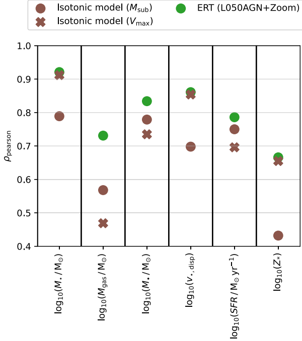
Figure B2. Pearson correlation coefficient for the ERT model (L050AGN + ZoomAGN) as well Isotonic regression models trained using subhalo mass and V_{\max} . Each predictor is shown on the x -axis.
