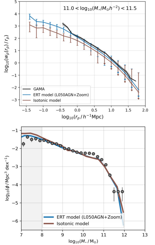
Figure B3. Predictions for the projected correlation function (top panel) and GSMF (bottom panel) using the Isotonic regression model (using subhalo mass; brown lines), compared with the ERT model (blue) with all features.
