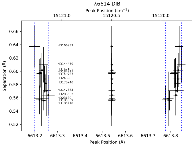
Fig. 5. Measured peak positions of the \lambda 6614 DIB in our target sightlines. Positions have been shifted such that the Q-branch lies at 6613.54 Å in all lines of sight.
