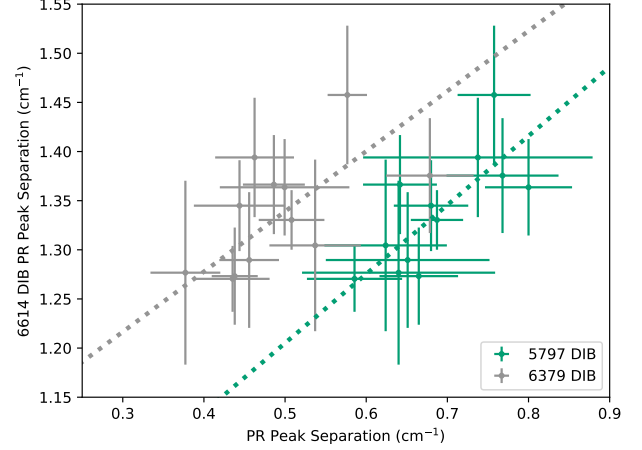
Fig. 4. P - to R -branch separation in all sightlines of the \lambda 6614 DIB (vertical axis) as a function of the separation of the \lambda 5797 (green) and \lambda 6379 (grey) DIBs on the horizontal axis (data values are listed in Table 2). The dotted lines are linear models of the data using orthogonal-distance fitting of the 6614 measurements as a function of the 5797 values (green) and 6379 values (grey).
