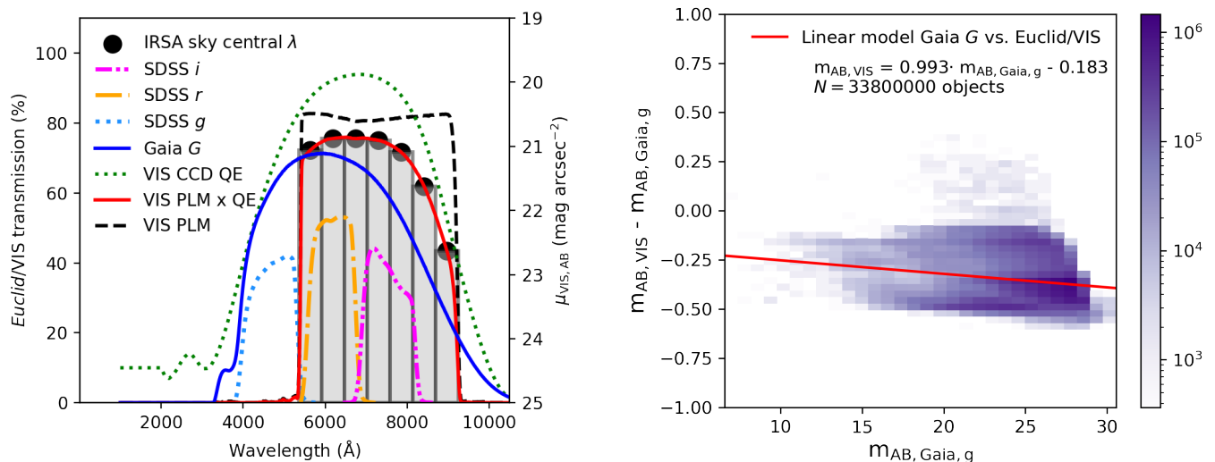
Fig. 2. Left panel: Solid red line: Euclid /VIS transmission curve. Solid blue line: Gaia G -band transmission curve (Venancio et al. 2020). Black dashed line: Euclid /VIS payload module (PLM) transmission curve. Green dotted line: Quantum Efficiency of the Euclid /VIS CCD detectors (including End of Life contamination), derived from initial engineering models. Grey columns: Wavelength ranges for the numerical integration of the transmission of VIS using the IRSA sky background model. Light-blue dotted line: SDSS g -band sensitivity for extended sources with zero airmass. Orange dash-dotted line: Equivalent for SDSS r -band. Magenta dash-dot-dotted line: Equivalent for SDSS i -band. Right panel: Euclid /VIS magnitude as a function of the Gaia G -band AB magnitudes for the synthetic stellar objects of the Euclid True Universe simulation. See the legend for the fitted linear transformation model between both bands.
