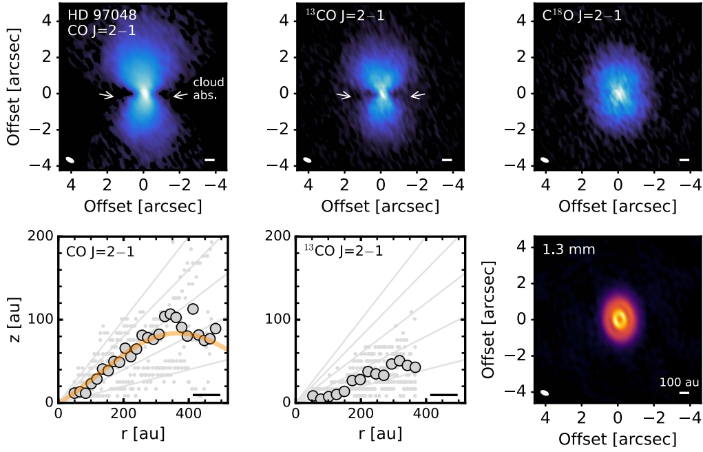
Figure 16. From left to right, top to bottom: CO, ^{13}\text{CO} , and \text{C}^{18}\text{O } J=2-1 zeroth moment maps; CO and ^{13}\text{CO} line emission surfaces; and 1.3 mm continuum image. The synthesized beam and a scale bar indicating 100 au are shown in the lower left and right corners, respectively, of each image. Regions of cloud contamination in the CO and ^{13}\text{CO } J=2-1 lines are marked with arrows. Large gray points show radially binned surfaces and small, light-gray points represent individual measurements. The orange line in the CO emission surface shows the exponentially tapered power-law fit (Table 2).
