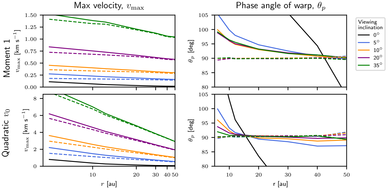
Figure 8. The velocity and warp phase angle measurement when disc is viewed at an inclination for the 10^\circ binary inclination warped disc (solid lines) and the unwarped aligned disc (dashed lines). The velocity maps were spatially deprojected first but no Keplerian subtraction is applied.
