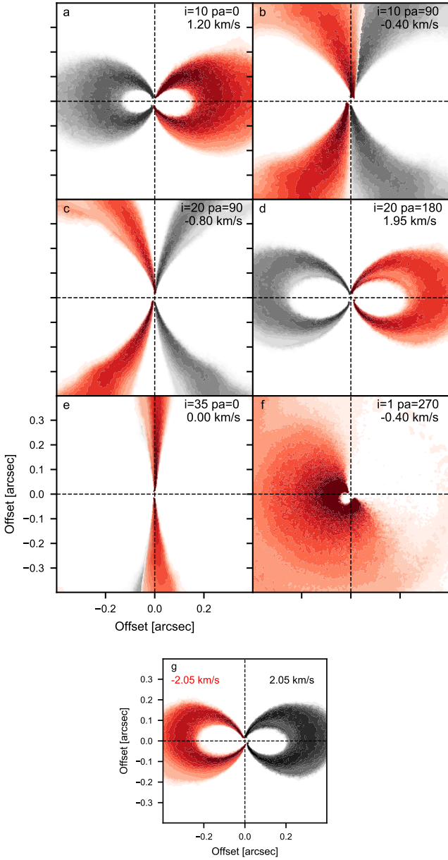
Figure 12. Continuum-subtracted channel maps for the 10° binary inclination model at various viewing inclinations and position angles (red shading). The corresponding channel maps of the aligned disc model are shown in grey (except panel f), reflected along the vertical axis for comparison to highlight the asymmetries in the emission from the warped disc. Panel g shows two channel maps from i=20 , pa=180 . Here we see asymmetry between opposite velocity channels. The back side of the disc is just detected at positive velocities (red) but not at negative velocities (grey).
