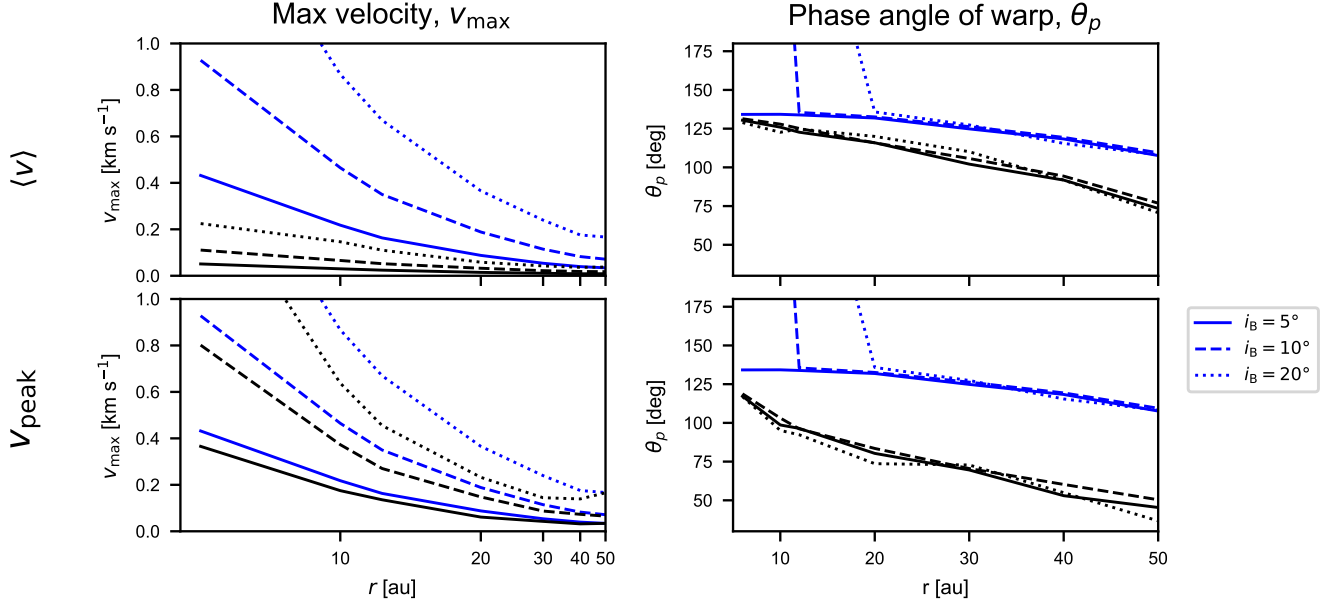
Figure 4. v_{\text{max}} and \theta_p profiles for models with initial misalignments of 5, 10 and 20^\circ of the binary to the disc after 1350 orbits. The profiles in the top row were derived from first moment maps and the profiles in the bottom row were derived from v_{\text{peak}} maps. Blue lines indicate results from the SPH output and black lines are results derived from the simulated ^{13}\text{CO} maps.
