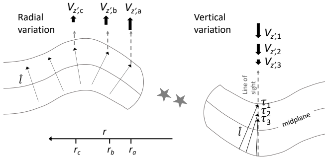
Figure 6. Sketch diagram to explain the observed CO velocities. The left hand side illustrates the radial variation of the line-of-sight velocity v_z , at r_a , r_b and r_c . The right hand side shows the vertical variation of v_z , which will be evident in tracers of differing optical depths \tau_i . The gas velocity is perpendicular to \hat{l} , the local specific angular momentum unit vector. Thin arrows indicate the orientation of \hat{l} and solid arrows indicate the magnitude of the observed tangential velocity. The angular momentum vector becomes more aligned with the the line of sight deeper into the disc. Shallower layers therefore have a greater tangential velocity and greater line-of-sight velocity.
