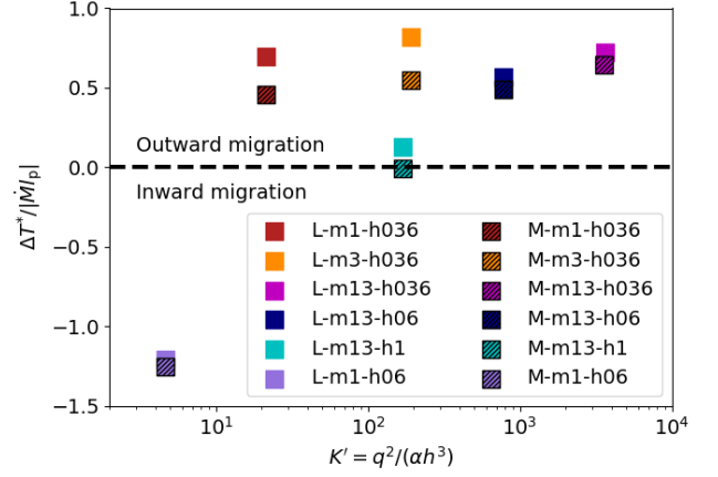
Figure 6. Torques associated to the rate of change of semi-major axis normalised for the VSS accretion rate times the local specific angular momentum as a function of parameter K' = q^2/(\alpha h^3) . The different colours correspond to different simulations, as indicated in the legend.
