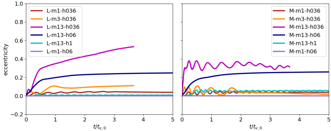
Figure 2. Eccentricity as a function of the evolutionary time for light disc simulations (left panel) and massive disc simulations (right panel). The different colours correspond to different simulations, as indicated in the plot legend (see Table 1 for the simulations' name definition).
