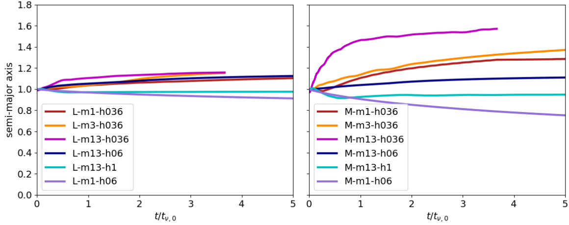
Figure 1. Semi-major axis as a function of the evolutionary time for light disc simulations (left panel) and massive disc simulations (right panel). The different colours correspond to different simulations, as indicated in the plot legend (see Table 1 for the simulations' name definition).
