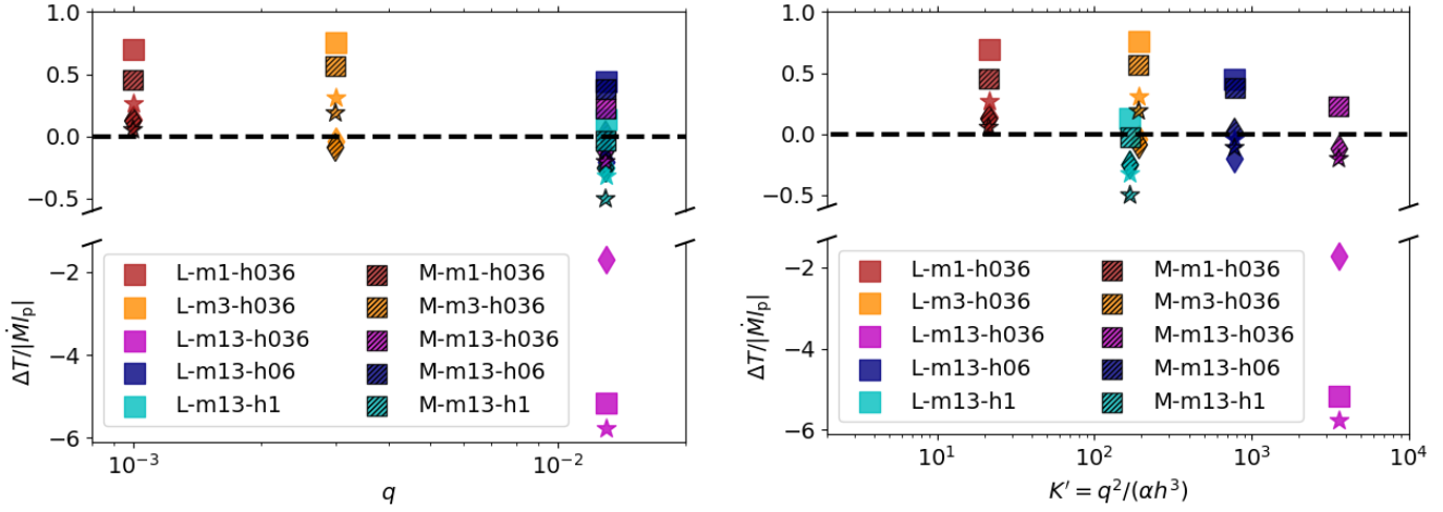
Figure 9. Torque acting on the planet normalised for the VSS accretion rate times the local specific angular momentum as a function of q (left panel) and parameter K' = q^2/(\alpha h^3) (right panel). The diamonds indicate the results from the open boundary condition simulations; the squares illustrate the torque the results from the viscous boundary condition simulations; the stars show the prediction for the open boundary condition results, applying Equation 16 to the results obtained from viscous boundary conditions.
