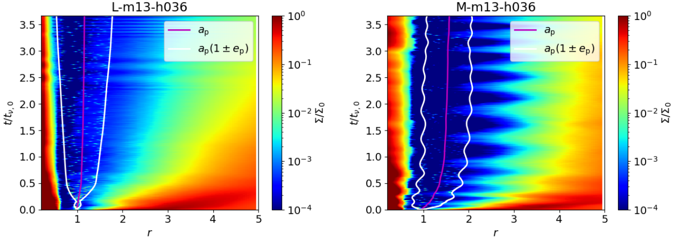
Figure 4. Azimuthal averaged density profiles \Sigma/\Sigma_0 (colour map) as a function of the radius ( x axis) and time normalised to the viscous timescale at the initial planet location ( y axis). The magenta line shows the time evolution of the planet’s semi-major axis; the white lines show the time evolution of a_p(1 \pm e_p) . The left panel refers to simulation L-m13-h036; the right panel refers to simulation M-m13-h036.
