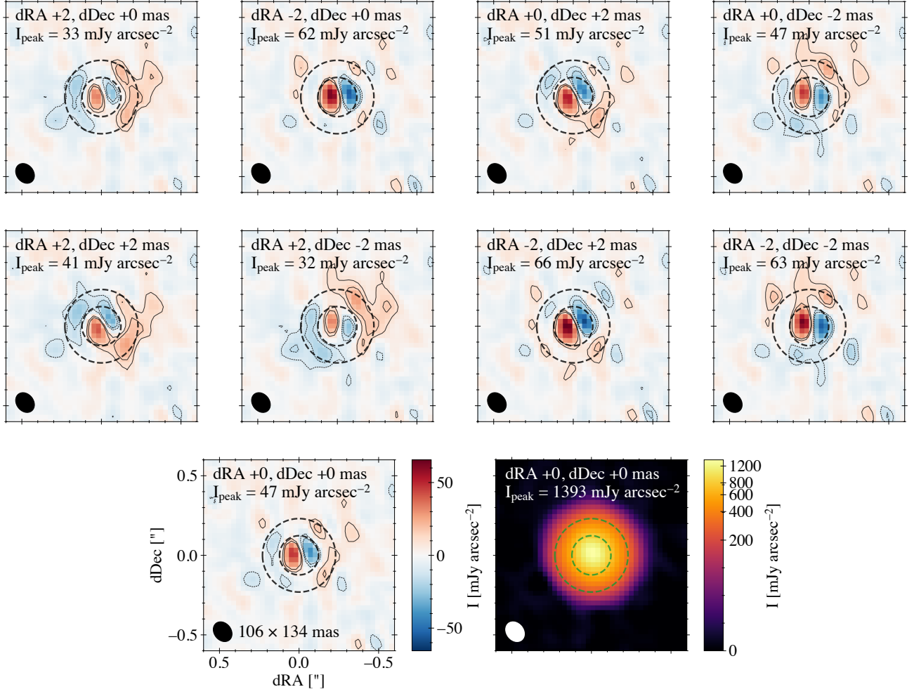
Figure A1. Effect of fitted phase center on imaged residual visibilities
