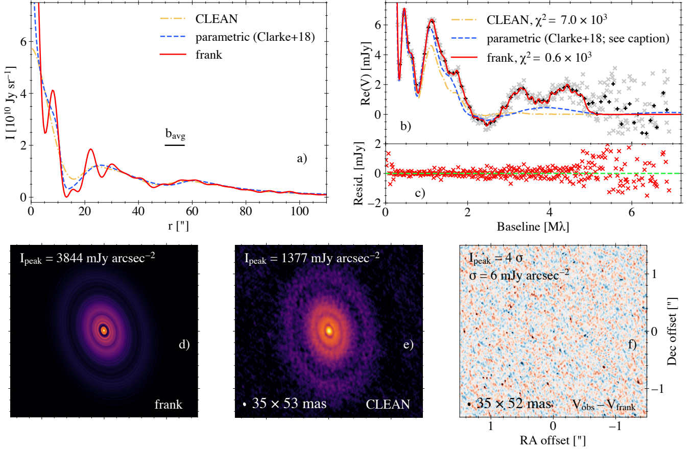
Figure C1. frank fit to high resolution CI Tau observations
