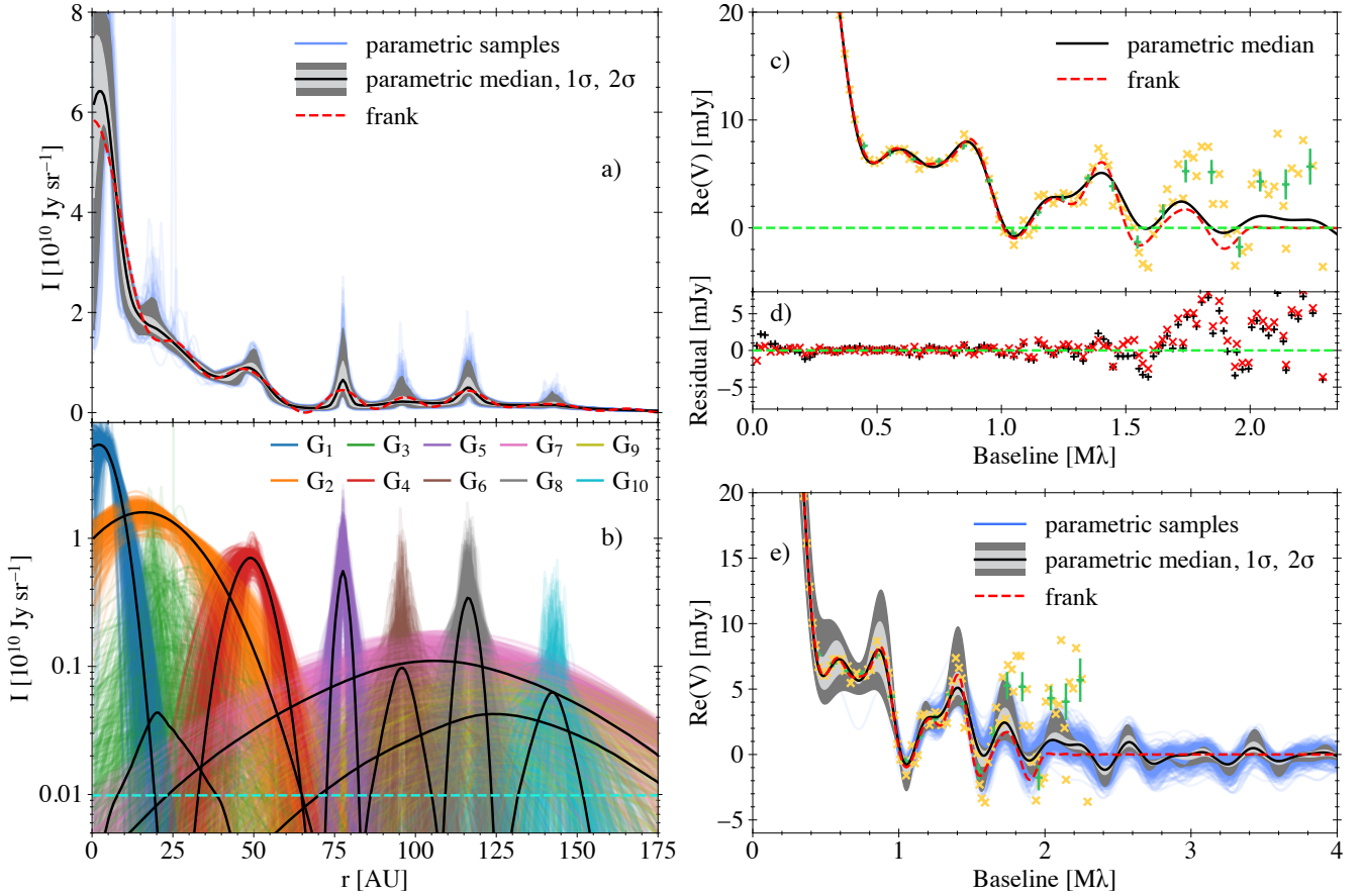
Figure 10. Ten Gaussian parametric fit to DL Tau
