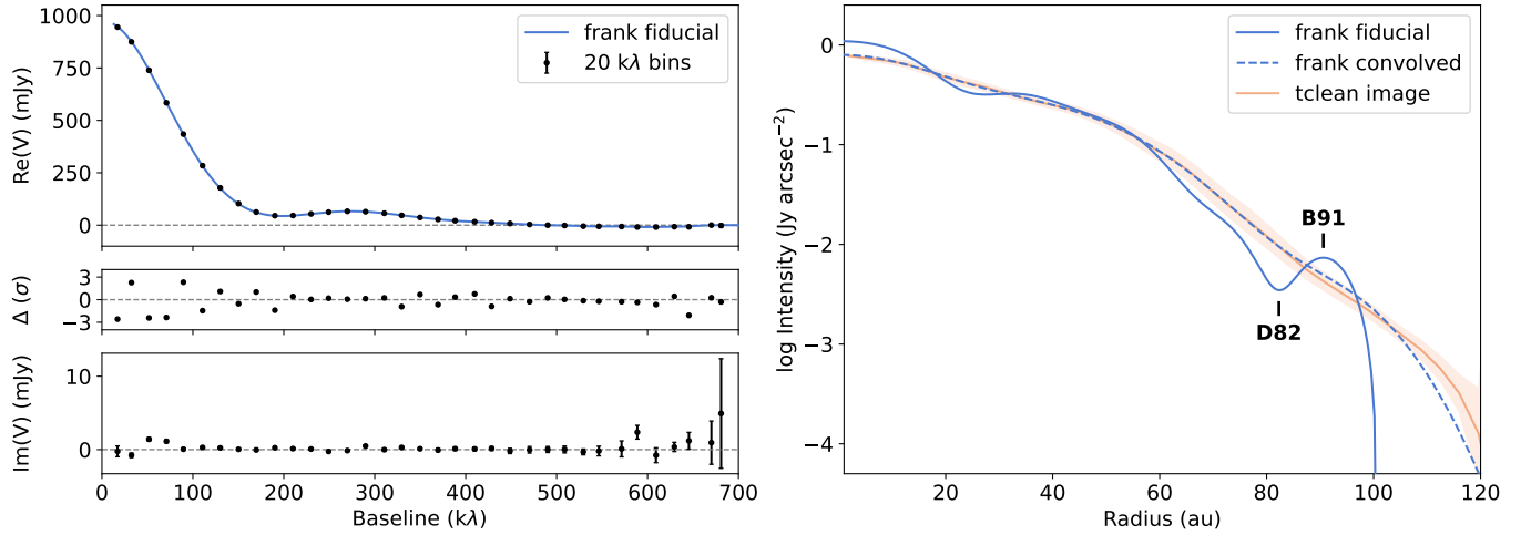
Figure 1. Left: Our fiducial frank fit compared to the real component of the visibilities \text{Re}(V) shown in 20 k \lambda bins. The lower panels show the residuals between fit and data ( \Delta ) in terms of the uncertainty on the weighted mean \sigma , and the imaginary component \text{Im}(V) . Right: The radial intensity profile derived from our fiducial frank fit (solid blue) shown alongside the intensity profiles of the deprojected tclean image (orange) and the fiducial frank fit convolved with the tclean beam (dashed blue). Shaded regions give the standard deviation for each bin. The newly identified dark gap (D82) and bright ring (B91) are marked.
