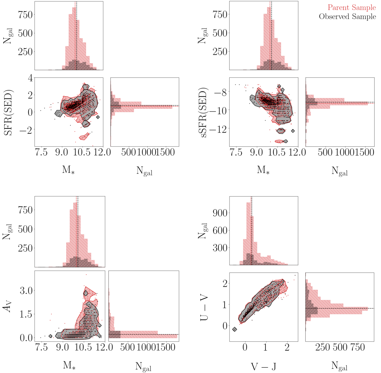
Figure 9. Corner plots for \text{SFR}(\text{SED}) , M_* (upper left), \text{sSFR}(\text{SED}) vs. M_* (upper right), A_V vs. M_* (bottom left), and U-V vs. V-J (bottom right). Shown on these diagrams are the z \sim 2 parent sample (red) and z \sim 2 observed sample (black). The galaxy properties shown here are estimated using emission-line uncorrected photometry for all galaxies in the figure. The parameter distributions and sample medians are shown in the 1D histogram panels, while the individual data points and 3\sigma shaded contours for each sample are shown in 2D space.
