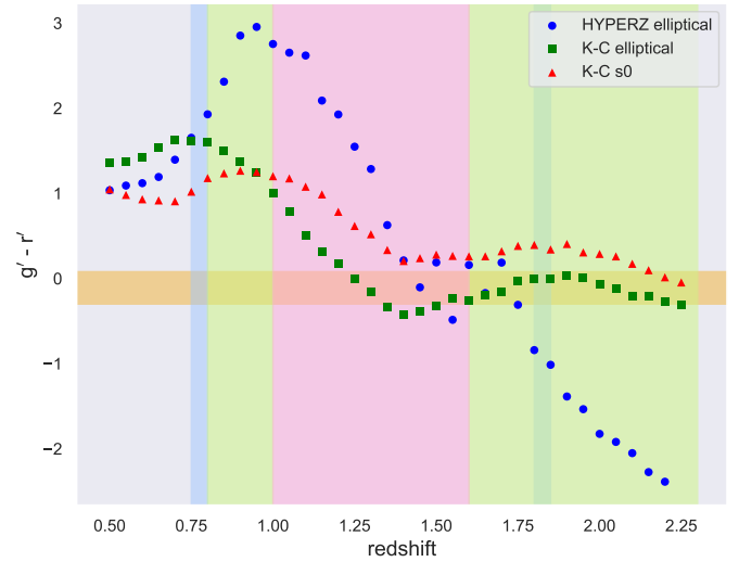
Figure 11: The g' - r' colour as a function of redshift ( z < 2.3 ) for the three template elliptical SEDs. Blue dots, green squares and red triangles represent the g' - r' colour for the HYPERZ CWW_E_ext.sed, and the elliptical_template and s0_template from the Kinney-Calzetti spectral atlas, respectively. Vertical light blue, light green (elliptical_template) and pink (s0_template) shaded regions indicate the redshifts of interest for elliptical galaxies obtained using HYPERZ and Kinney-Calzetti spectral atlas SEDs (see Figure 10). Given that the redshift ranges for the HYPERZ and elliptical_template overlap partially the vertical bar around redshift 1.80–1.85 has an undetermined colour. The horizontal dark yellow shaded region shows the 1\sigma colour uncertainty for the host candidate cNW, respectively. There is no redshift region where the combined colour and size–luminosity constraints overlap for the HYPERZ and the s0 Kinney-Calzetti templates. Only for the elliptical Kinney-Calzetti template the combined constraints agree to within 1\sigma for a redshift in the range of 1.6–2.3.
