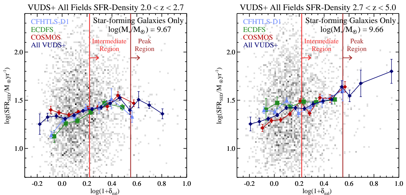
Fig. 7. The redshift dependence of the SFR - \delta_{gal} relation in the VUDS+ sample. The two panels are identical to the left panel of Figure 5 except now the VUDS+ sample is broken up into two redshift bins with approximately equal numbers of galaxies. The meaning of the points and their associated uncertainties are identical to those in Figure 5 as are the meanings of the vertical lines. As in Figure 5, the SFR - \delta_{gal} for all three VUDS+ fields are shown along with the combined sample. The left panel shows the SFR - \delta_{gal} relation for the lower-redshift sample ( 2.0 \leq z \leq 2.7 ) and the right panel shows the relation for the higher-redshift sample ( 2.7 < z \leq 5.0 ). The average stellar mass of each sample is given in the top-right portion of each panel and is effectively identical between the two samples. While a significant positive correlation between SFR - \delta_{gal} exists in the lower-redshift sample, this correlation disappears when considering only galaxies in the Intermediate and Peak regions. In contrast, in the higher-redshift bin, the significant positive correlation is seen at all environments and increases in strength in the densest regions.
