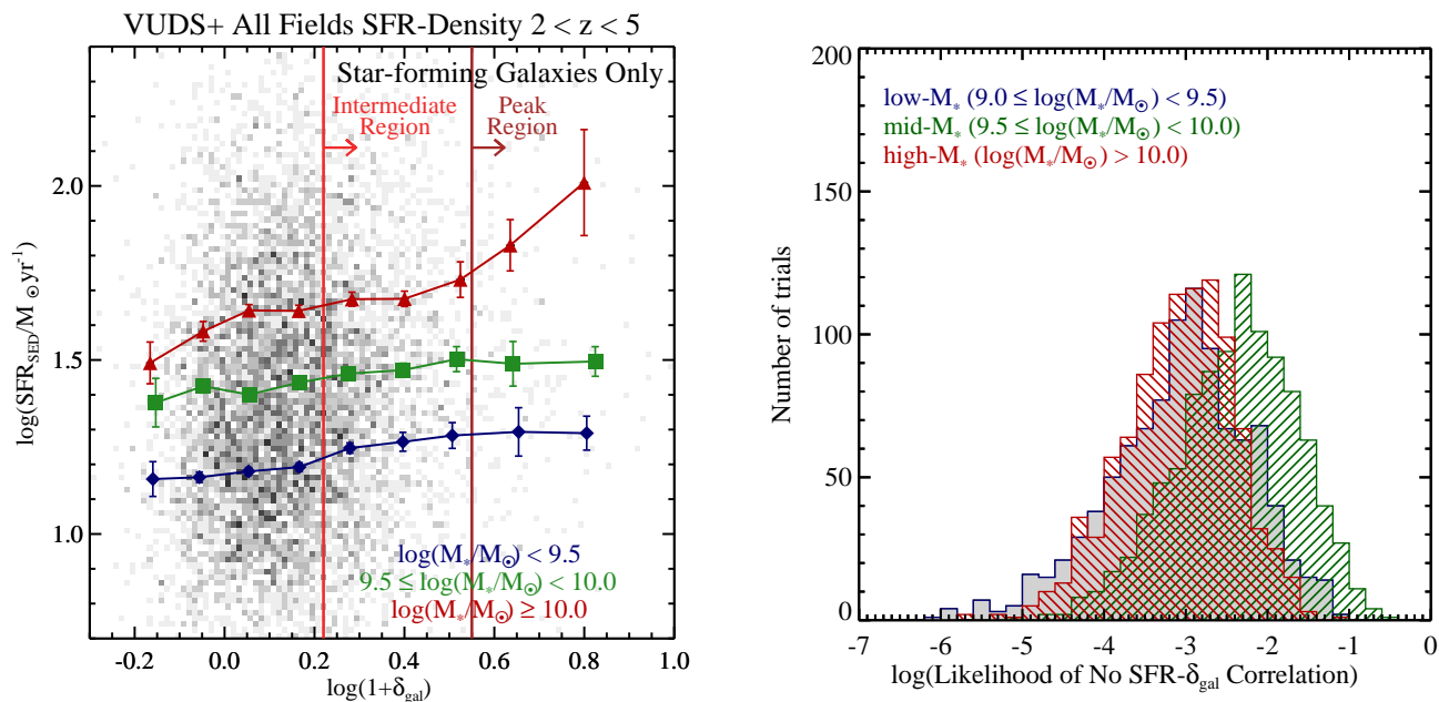
Fig. 6. The SFR -density relation in the VUDS+ sample as a function of stellar mass. Left: As in the left panel of Figure 5, the SFR - \delta_{gal} relation for our final VUDS+ sample, but now with galaxies broken up into three approximately equally-sized samples binned in stellar mass using the limits indicated at the bottom right of the panel. The points and their associated uncertainties have the same meaning as in Figure 5. The solid vertical lines and their meanings are the same as in Figure 5. A weak but significant positive correlation between SFR and \log(1 + \delta_{gal}) is seen in the two lower mass bins. A stronger and equally significant positive correlation is seen for the highest stellar mass galaxies and is especially apparent in the Peak Region. Right: Distribution of the logarithmic value of the likelihood of no correlation between SFR and \log(1 + \delta_{gal}) of our final spectral sample for the three different stellar mass bins used in our analysis for the full redshift range 2 \leq z \leq 5 . This distribution is calculated from 1000 Monte Carlo realization in which we perturb each SFR and \log(1 + \delta_{gal}) value by their associated errors. These histograms do not meaningfully change if we additionally include dusty star-forming galaxies with high rates of SFR and galaxies with no active star formation, both of which are completely missed in our sample, at proportions appropriate for their number density at 2 \leq z \leq 5 in our Monte Carlo simulations. For reference, a \log(\text{likelihood}) < -2.5 corresponds to a positive correlation between the two parameters estimated at \geq 3\sigma confidence level.
