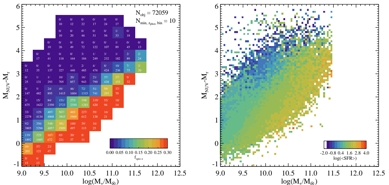
Fig. 9. Color, stellar mass, and SFR properties of the VUDS+ spectroscopic and parent photometric sample. Left: Rest-frame color-stellar mass diagram of an observed-frame NIR-selected sample of z_{phot} and z_{spec} objects in across the three VUDS fields. The fraction of z_{phot} objects with a secure spectral redshift in each color/stellar mass bin is indicated by the color bar. In each color/stellar mass bin the number of z_{spec} and z_{phot} objects are given by the upper and lower number in each box, respectively. Only those bins that contained ten or more z_{phot} objects are plotted. This plot is nearly identical to the right panel of Figure 4, but here the bins are coarser to reflect the size used to perform the weighted Monte Carlo SFR-\delta_{gal} analysis presented in this section. Right: Color-stellar mass diagram of the z_{phot} sample plotted in the left panel with the color bar now corresponding to the average SED-fit SFR of all objects in that bin. No color or stellar mass limits are imposed on the galaxies plotted here, and two-dimensional bins are now plotted if they contain at least one object. The average SFR is seen to vary smoothly as a function of color and stellar mass over the range plotted. While the clear preference of the VUDS+ spectral sampling toward bluer galaxies at fixed M_* appears to potentially bias the spectral sample to higher SFR s, from the analysis presented in this section we conclude that this potential bias does not drive the significant positive correlation between SFR and \delta_{gal} seen in the full VUDS+ sample.
