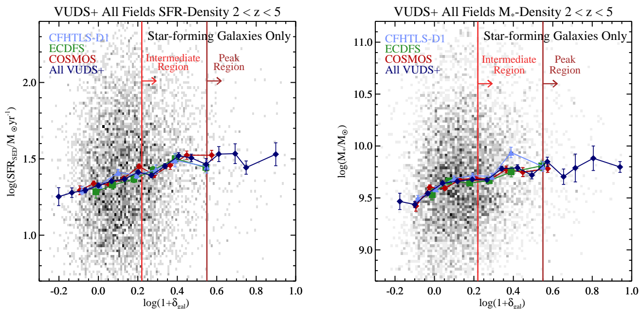
Fig. 5. Galaxy properties as a function of environment in the VUDS+ sample. Left: Relationship between SFR and \log(1 + \delta_{gal}) for the 6730 galaxies in the VUDS+ spectroscopic sample. The backdrop shows the number density at a given SFR and \log(1 + \delta_{gal}) value for all galaxies in the sample and the light blue, green, red, and dark blue datapoints and lines show median values in each bin in \log(1 + \delta_{gal}) for galaxies in the CFHTLS-D1, ECFDS, COSMOS, and the full combined VUDS+ sample, respectively. The vertical dashed lines indicate the “Intermediate” and “Peak” regions of the \log(1 + \delta_{gal}) distributions (see §3.1), with all values lower than \log(1 + \delta_{gal}) = 0.22 being considered “Field” galaxies. The “All VUDS+” sample can be plotted over a larger dynamic range in \log(1 + \delta_{gal}) relative to the individual field samples due to its larger sample size. A weak but highly significant positive correlation is observed (see §3.1). Right: As in the left panel, but now plotted for stellar mass ( M_* ) and \log(1 + \delta_{gal}) . Again, a weak but highly significant positive correlation is observed between M_* and \log(1 + \delta_{gal}) .
