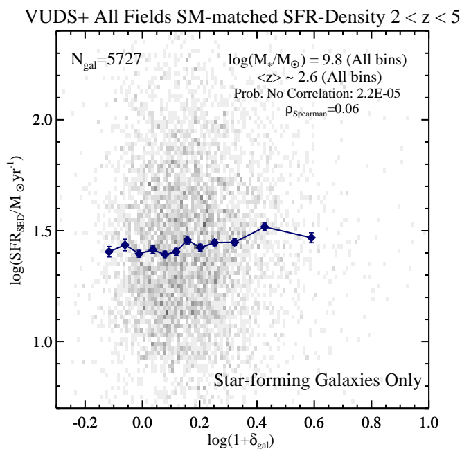
Fig. 8. Relationship between SFR and \log(1 + \delta_{gal}) for a stellar-mass and redshift-matched sample of galaxies. Each bin in \log(1 + \delta_{gal}) originally contained 10% of the final VUDS+ sample. Galaxies in each decile were clipped in order to have the same median redshift and stellar mass within the uncertainties with every other decile. The bins in the lower and upper decile of the \log(1 + \delta_{gal}) distribution were cut in half for illustrative purposes. The approximate median stellar mass and redshift of all bins is indicated in the top right and the number of galaxies remaining in the sample indicated in the top left. The data points and their associated uncertainties were calculated in the same way as Figure 5. In the top right of the plot the Spearman’s correlation coefficient for this sample and the likelihood of no correlation are shown. Despite normalizing by stellar mass and redshift, a weak but significant positive SFR - \delta_{gal} trend is observed.
