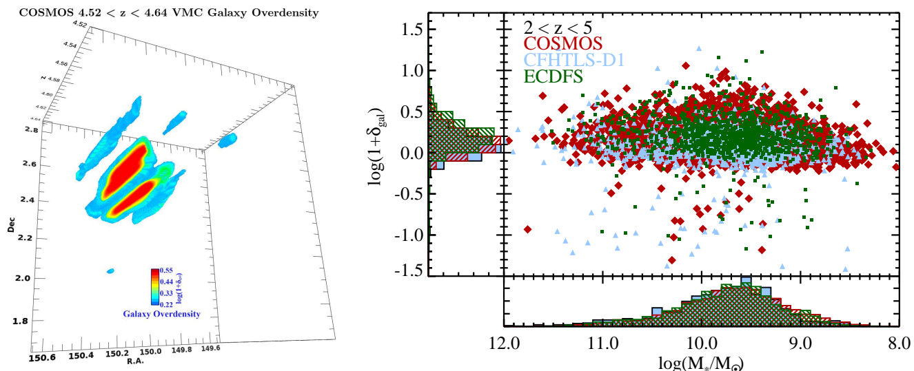
Fig. 2. Galaxy overdensity reconstruction using the VMC mapping method. Left: Example of our VMC overdensity mapping (see §2.4) as applied to the COSMOS field in the redshift range 4.52 \leq z \leq 4.64 , nearly an identical range as is shown in Figure 1. The main structure seen in the mapping is again the PCI J1001+0220 proto-cluster at z \sim 4.57 . Here, in addition to showing the transverse dimensions, we also show the extent of the structure in the third dimension, redshift, which extends in this cube between 4.52 \leq z \leq 4.64 . The redshift dimension is added by rendering the narrow redshift slices used in our analysis to define galaxy overdensity rather than employing a single slice over the redshift extent of the proto-cluster as was done in Figure 1. The scale bar in the lower right shows the galaxy overdensity values, with the lower and upper end of the dynamic range corresponding the “Intermediate” and “Peak” regions as defined in §3.1. Right: Distribution of the full VUDS+ spectral sample in M_* and \log(1 + \delta_{gal}) for the three separate fields targeted by VUDS (ECDFS: small green squares, CFHTLS-D1: light blue triangles, COSMOS: large red diamonds). The redshift range imposed on the plotted galaxies is shown in the top left. Area-normalized histograms for the three fields for both parameters are shown on the side of the plot. The three fields show generally similar distributions in both parameters, with a slight excess of galaxies at higher \log(1 + \delta_{gal}) observed in COSMOS and ECDFS.
