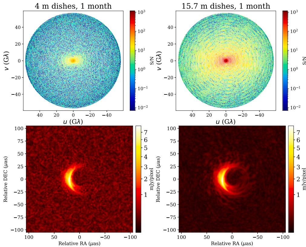
Fig. 1. Top: Signal-to-noise ratio of individual visibilities (integration times 0.5–7.5 min depending on baseline length) when observing a GRMHD model of Sgr A* [model 39 from [14]] at 690 GHz with the Event Horizon Imager (EHI) system, using system noise parameters from [15] and three dishes with a diameter of 4 (left) or 15.7 (right) m. Bottom: images reconstructed by taking an FFT of the visibilities on a 116 \times 116 pixel grid. The normalised cross-correlation when comparing to the average image of the observed movie is 0.89 and 0.97 for 4 and 15.7-meter dishes, respectively.
