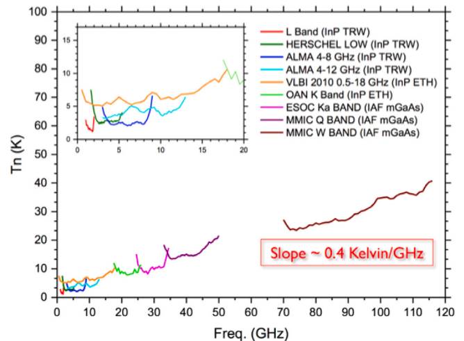
Fig. 10. Noise temperature (at T_{\text{amb}} = 15 K) and frequency coverage of various amplifiers developed at Yebes Observatory. These amplifiers are used for either type of heterodyne receivers, some designs for both. The amplifiers above 20 GHz are used only in direct amplification heterodyne receivers, while the lower frequency ones (inset) are used also as IF amplifiers for the THz range.
