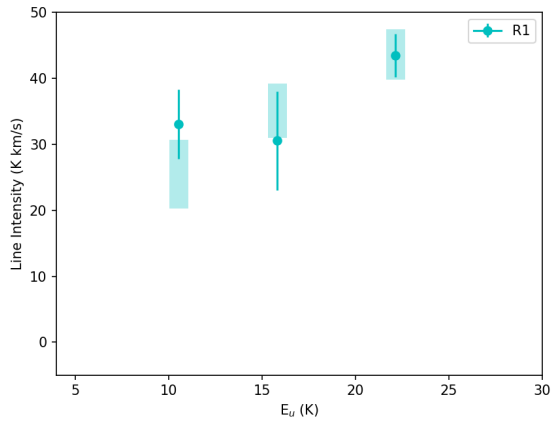
(a) Observed and PPC intensities of HCNCO in CND-R1
