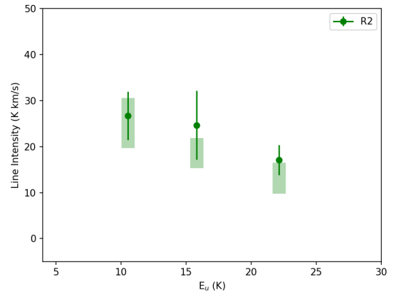
(b) Observed and PPC intensities of HCNCO in CND-R2
