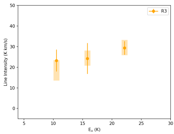
(c) Observed and PPC intensities of HCNCO in CND-R3
