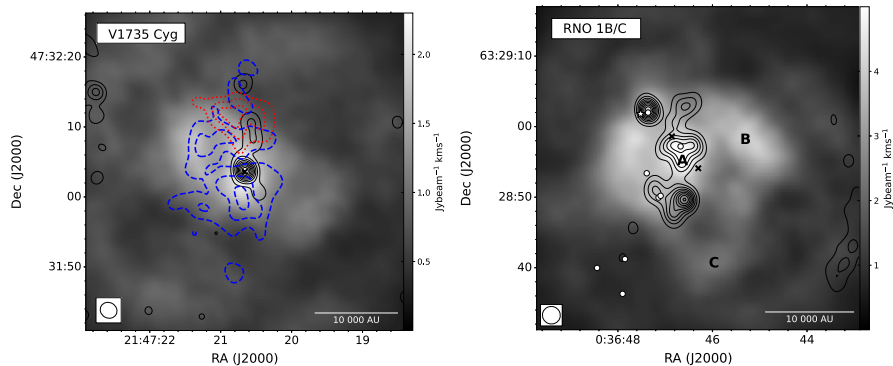
Figure 1. NOEMA CO and continuum maps of northern FUors (adapted from [7] and [8]). Left: ^{13}\text{CO} integrated intensity map of V1735 Cyg. The cross marks the optical position of the FUor, the black contours are the 2.7 mm continuum emission in units of \text{Jy beam}^{-1} at the 10...90% of the peak. The dashed contour is the blue-shifted (integrated between -0.2 – 2 \text{ km s}^{-1} ) and the dotted contour is the red-shifted lobe (integrated between 7 – 9.4 \text{ km s}^{-1} ) of the outflow at 50, 70 and 90% of their peak emission. Right: ^{13}\text{CO} integrated intensity map of RNO 1B/C. The black contours are the 2.7 mm continuum emission at the 10...90% of the peak. The two crosses are the members of the binary FUor-system (RNO 1B is at the center) and the star symbol marks an IRAS source. The letters mark clumps identified on the CO map and circles mark some of the other IR/sub-mm/mm sources in the vicinity.
