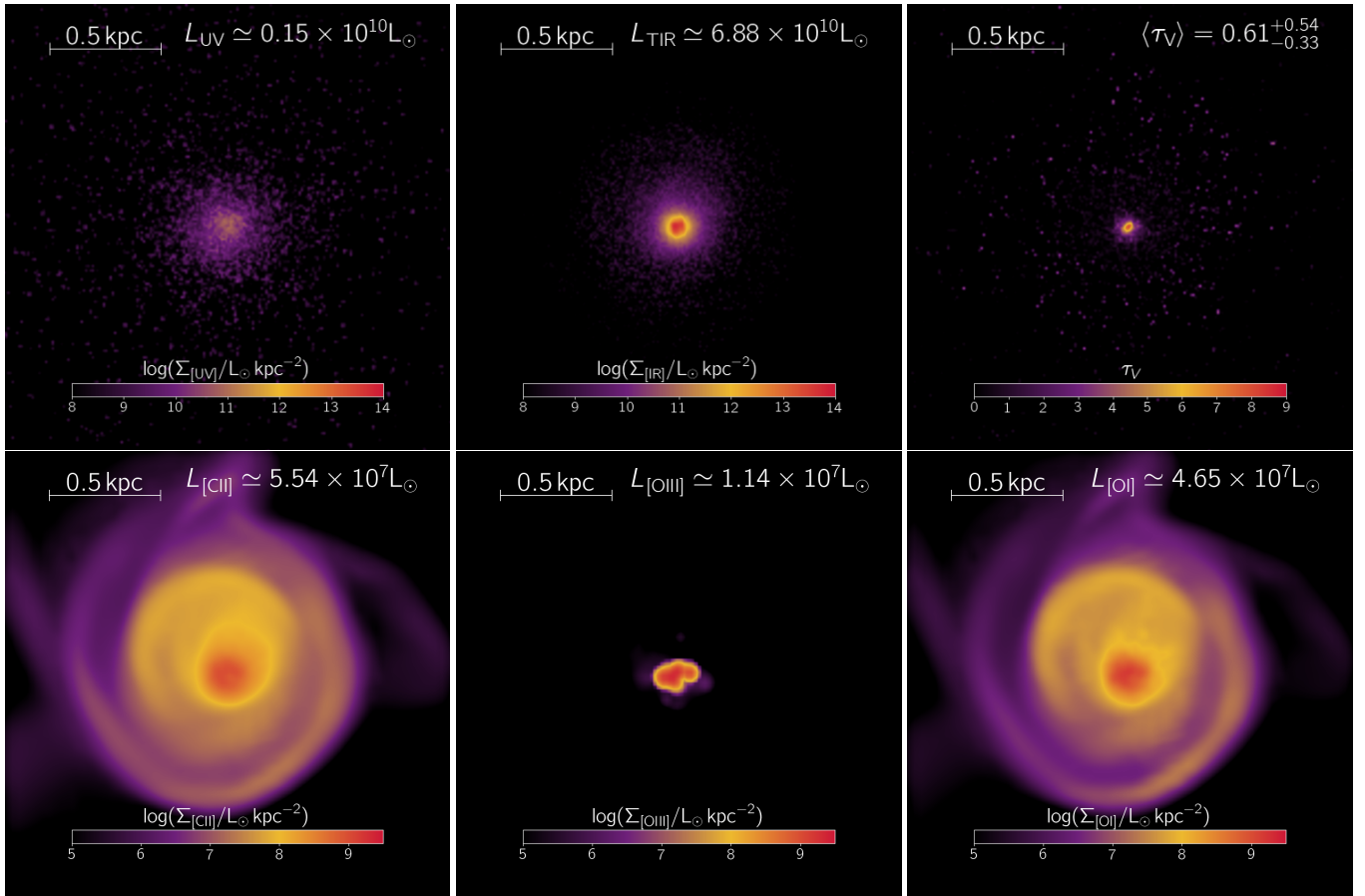
Figure 8. Emission properties of “Dianthus”, a M_{\star} = 2.53 \times 10^9 M_{\odot} star forming galaxy in SERRA ( z = 7.7 ). The upper panels show the continuum properties: the surface brightness in the restframe UV ( left , \Sigma_{UV} , 1000 \leq \lambda/\text{\AA} \leq 3000 ) in the total IR emission ( center , \Sigma_{TIR} , 8 \leq \lambda/\mu\text{m} \leq 1000 ), and the V-band optical depth ( right , \tau_V ). The lower panels show the surface brightness of a set of FIR emission lines: [C II] ( left , 158\mu\text{m} ), [O III] ( center , 88\mu\text{m} ), [O I] ( right , 61\mu\text{m} ). The maps are taken in a FOV of 2 kpc with a face-on orientation. As insets, we report the total luminosity of each emission map and the average value of \tau_V . Models for line and continuum emission are described in Sec.s 2.4.2 and 2.4.3, respectively.
