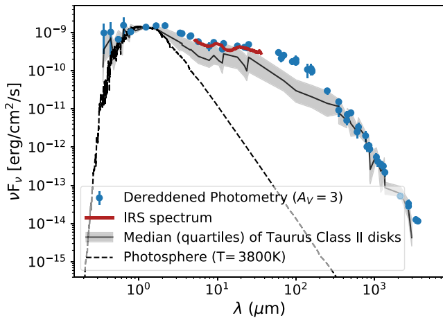
Figure 15. A comparison between the spectral energy distribution of DO Tau and other Class II disks in Taurus. The blue points (with 1\sigma error bars) denote dereddened photometric measurements presented in Andrews et al. (2013) and Ribas et al. (2017). An A_V value of 3 is adopted based on Andrews et al. (2013). The red curve corresponds to the Spitzer/IRS spectrum retrieved from the Cornell Atlas of Spitzer/IRS Sources (Lebouteiller et al. 2011, 2015). The dashed black curve shows the estimated stellar photosphere. The solid black curve corresponds to the median dereddened Taurus Class II SED from Ribas et al. (2017), while the gray shaded area corresponds to the interquartile range.
