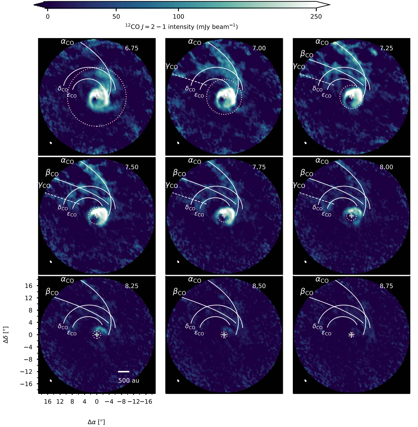
Figure 12. ^{12}\text{CO } J = 2 - 1 channel maps annotated in white with the locations of the \alpha_{\text{CO}} , \beta_{\text{CO}} , \gamma_{\text{CO}} , \delta_{\text{CO}} , and \epsilon_{\text{CO}} streams. The \gamma_{\text{CO}} feature is marked with a dashed line rather than a solid line because its identification is less certain. The dotted pink circle denotes the radius at which the line-of-sight velocity relative to DO Tau is equal to the escape velocity. The LSRK velocity ( \text{km s}^{-1} ) appears in the top right of each panel. The synthesized beam is shown as a solid white ellipse in the lower-left corner. A gray cross marks the position of the millimeter continuum peak, which is located at the phase center. Offsets from the phase center (in arcseconds) are marked in the lower-left panel. The top end of the color bar is saturated in order to show the faint extended features in more detail. North is up, and east is to the left.
