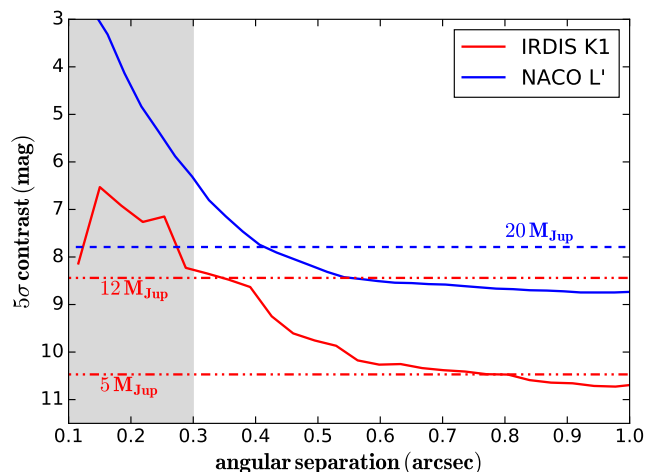
Fig. 5. Achieved contrast in the SPHERE K-band (red) and the NACO L-band (blue) observations. We indicate the contrast for 5 M_{Jup} and 12 M_{Jup} objects in K-band and a 20 M_{Jup} object in L-band. We used AMES-DUSTY models to convert the contrast to mass limits assuming a system age of 5 Myr. The grey shaded area marks the inner cavity of the scattered light disk inside of features A1 and A2.
