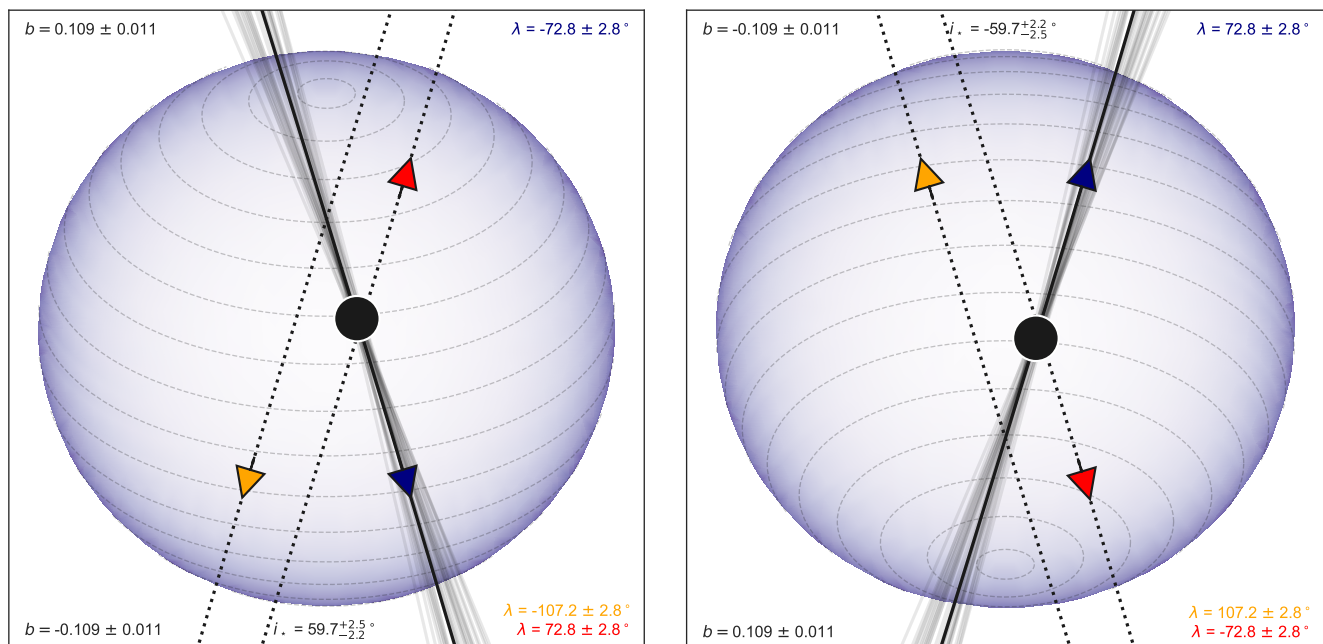
Fig. 6. Visualisation of the path of the MASCARA-1 b transit across the stellar disk using the CHEOPS + Spitzer fit with priors from Doppler tomography. The star rotates anti-clockwise when viewed from the top, and the majority of the hemisphere in view moves from left to right. Constant stellar latitudes are marked with curved dashed lines. The colour scale is proportional to the flux emitted by the star, with brighter areas marked with lighter colours. For a given i_* , all possible transit paths of the planet across the star can be described using different combinations of b and \lambda . The \{b, \lambda\} pair associated with the median path transited by the planet is shown with a solid black line with a blue arrow indicating the direction, and with 32 samples drawn from the posterior shown in grey. The dashed lines with red and orange arrows indicate alternative \{b, \lambda\} pairs that also describe the signals in the Doppler tomography and transit light curves, respectively. However, when considering the tomography and the transit light curve together, only the \{b, \lambda\} pair described by the blue arrow can successfully describe them both. Assuming stellar symmetry about the equatorial plane, there are two indistinguishable solutions for each arrow in the range -90 < i_* < 90 deg: one with \{b, i_*, \lambda\} and another with \{-b, -i_*, -\lambda\} . The \{b, \lambda\} pairs with positive i_* (north pole pointing towards the observer) are shown in the left panel, and the \{b, \lambda\} pairs with negative i_* (north pole pointing away from the observer) are shown in the right panel. The blue arrow in the left panel is an example of a solution fitting the light curve with b > 0 , and -90 < \lambda < 90 deg, and corresponding solutions are found for all of the transit fits presented in this paper.
