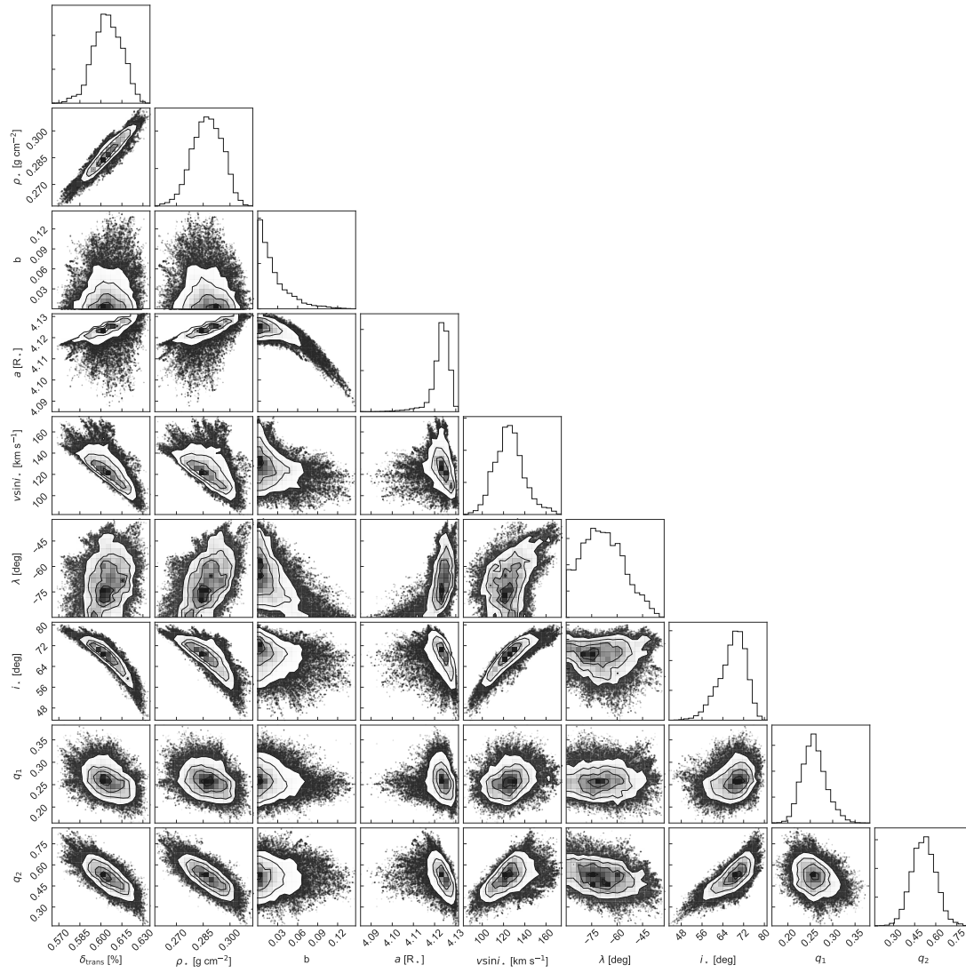
Fig. B.2. Corner plot of the CHEOPS+Spitzer transit-only fit without the placement of Gaussian priors on b , v \sin i_* , and \lambda informed by the Doppler tomography. The strategy is described in full in Section 5 and the corresponding results are displayed in Table 3.
