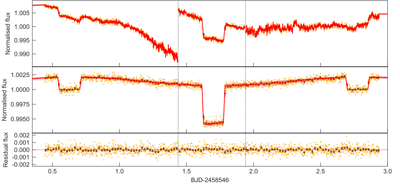
Fig. 4. Normalised flux associated with the Spitzer phase curve observation. The raw data are shown in orange points, and data in bins of 30 minutes are shown in brown points with error bars. The best fitting model is shown with a red line, and the 32 models evenly spaced in the chain are shown in fainter red lines. The times when a new AOR begins are marked with dashed vertical lines. The top panel shows the raw flux, the middle panel shows the flux corrected for the instrumental effects with the transit, occultations and phase variations, and the bottom panel shows the residual flux. The mean absolute deviation of the residuals is 244 ppm.
