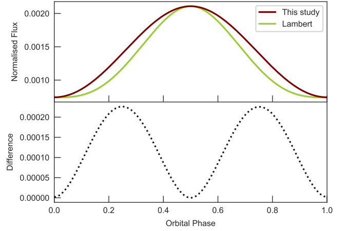
Fig. 10. Top panel: phase curve model associated with the median result for the Spitzer bandpass (maroon), which is the sum of the thermal and reflected light components described in Section 4.2. A Lambertian phase curve model with the same amplitude, minimum flux, and hotspot offset (green) is also shown. Bottom panel: flux difference between the two models.
