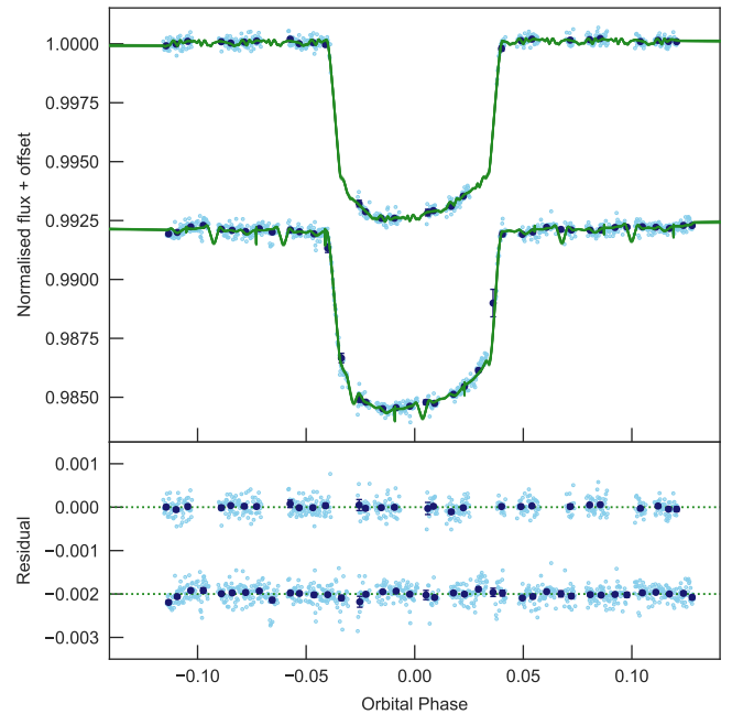
Fig. 1. Normalised flux associated with the two CHEOPS transit observations as a function of orbital phase, with an arbitrary offset applied for display purposes. The raw data are shown in light blue points, and data in bins of 12 minutes are shown in dark blue points with error bars. The best fitting model is shown with a green line, and the 32 models evenly spaced in the chain are shown in fainter green lines. The top panel shows the raw flux, and the bottom panel shows the residual flux. The asymmetry visible in the transits is caused by stellar rotation-induced gravity darkening. The root mean square (RMS) of the residuals is 365 ppm.
