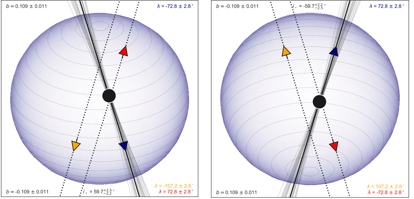
Fig. 6. Visualisation of the path of the MASCARA-1 b transit across the stellar disk using the CHEOPS + Spitzer fit with priors from Doppler tomography. The star rotates anti-clockwise when viewed from the top, and the majority of the hemisphere in view moves from left to right. Constant stellar latitudes are marked with curved dashed lines. The colour scale is proportional to the flux emitted by the star, with brighter areas marked with lighter colours. For a given i_* , all possible transit paths of the planet across the star can be described using different combinations of b and \lambda . The \{b, \lambda\} pair associated with the median path transited by the planet is shown with a solid black line with a blue arrow indicating the direction, and with 32 samples drawn from the posterior shown in grey. The dashed lines with red and orange arrows indicate alternative \{b, \lambda\} pairs that also describe the signals in the Doppler tomography and transit light curves, respectively. However, when considering the tomography and the transit light curve together, only the \{b, \lambda\} pair described by the blue arrow can successfully describe them both. Assuming stellar symmetry about the equatorial plane, there are two indistinguishable solutions for each arrow in the range -90 < i_* < 90 deg: one with \{b, i_*, \lambda\} and another with \{-b, -i_*, -\lambda\} . The \{b, \lambda\} pairs with positive i_* (north pole pointing towards the observer) are shown in the left panel, and the \{b, \lambda\} pairs with negative i_* (north pole pointing away from the observer) are shown in the right panel. The blue arrow in the left panel is an example of a solution fitting the light curve with b > 0 , and -90 < \lambda < 90 deg, and corresponding solutions are found for all of the transit fits presented in this paper.
