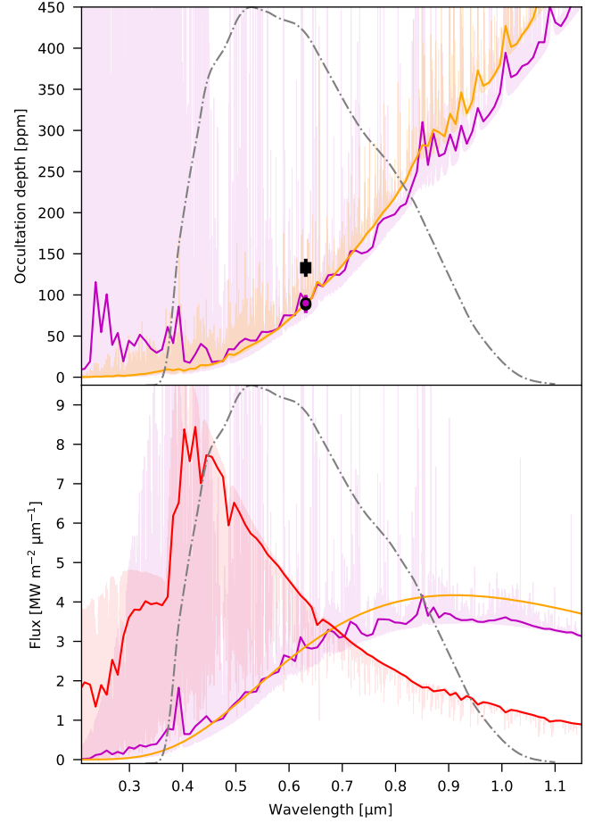
Fig. 12. Closer look at the emission spectra at wavelengths covered by the CHEOPS bandpass, enclosed by dotted lines in Fig. 11.
