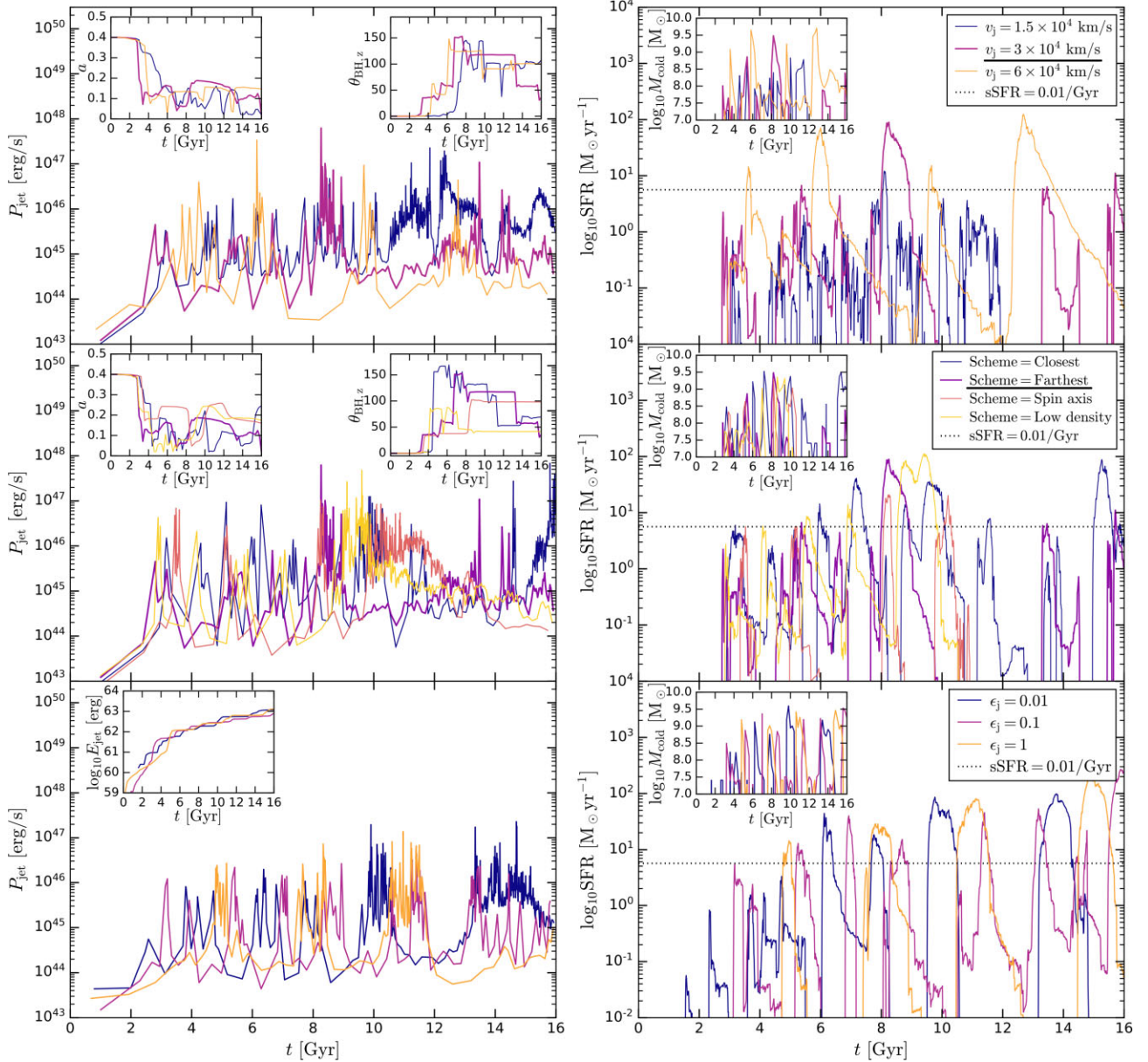
Figure 10. Time dependence of the quenching/feedback process in the high-mass galaxy cluster simulations ( M_{200} = 10^{15} M_{\odot} ) with varying parameters/choices, as per the legends in the right-hand panels. In the top row we vary the jet launching velocity, and in the middle row the choice of which particles are kicked from the SMBH smoothing kernel. The bottom row shows a case with the jets fixed along the z -axis, with the jet power calculated using a fixed efficiency (see legend). The left-hand panels show the jet power, while the right-hand panels show the star formation rate. Insets in the left-hand panels show the magnitude of SMBH spin and the angle between the spin vector and z -axis in the top and middle panel, and the total injected jet energy in the bottom panel. The insets in the right-hand panels show the cold gas mass. The details of the fiducial case, relative to which these variations are made, are given in Table 1 (purple line in each panel and underlined parameter in each panel legend, with the exception of the bottom row). The dotted black lines represent the upper limit of the specific star formation rate required to classify a galaxy as quenched.
