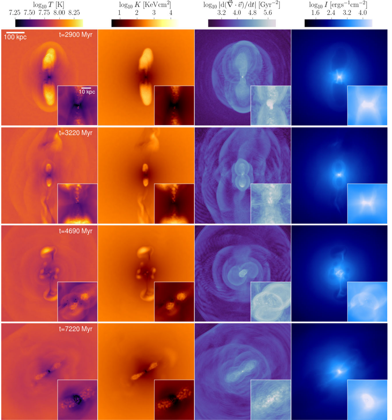
Figure 8. Gas properties (mass-weighted means) at different times in our fiducial simulation (see Table 1 for details) of the high-mass galaxy cluster ( M_{200} = 10^{15} M_{\odot} ). Each image is 800 kpc across, and shows slices 200 kpc in depth. Insets show a zoom-in of the central 50 kpc (10 kpc in depth). From left to right we show the temperature, entropy, shock/sound wave indicator and X-ray surface brightness (see the text for details). From top to bottom we show different times. The video version of the X-ray plots is available to view at https://youtu.be/113F4ndbm1c .
