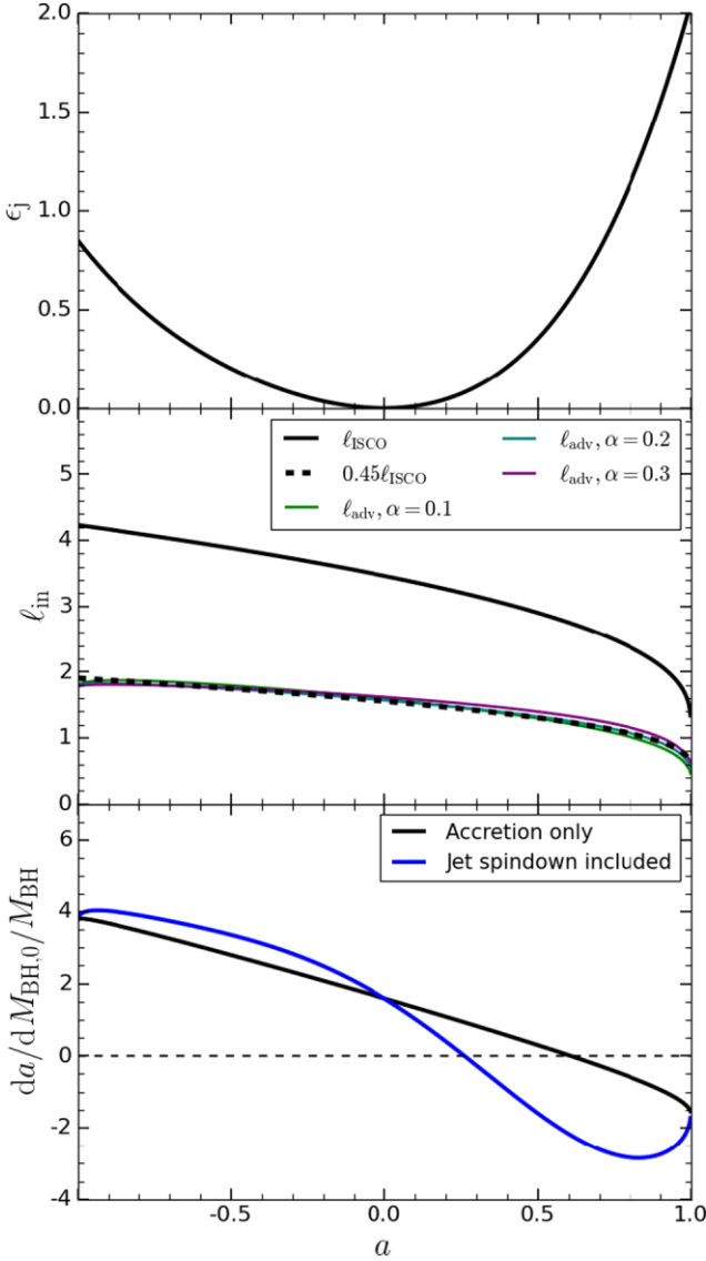
Figure 1. The dependencies on spin of the jet efficiency (top), (dimensionless) specific angular momentum at the inner radius (middle) and spin-up/spin-down function for thick, advection-dominated discs (bottom). The jet efficiency is given by equation (2). In the middle panel, coloured lines show the fitting function for the specific angular momentum of accreting matter from Benson & Babul (2009), for a few possible values of accretion disc viscosity \alpha . These are all approximately consistent with 45 per cent of the thin-disc specific angular momentum at the ISCO (innermost stable circular orbit, see the Online Appendix A for expression), for all spins. In the bottom panel, the black line (equation 5) shows that SMBHs surrounded by thick discs never spin-up beyond a = 0.6 , while the blue line (adding the equation 6 term) shows that jets bring this equilibrium spin value down to 0.25.
