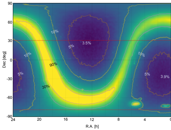
Fig. 12. Sky coverage for laser guide star adaptive optics supported off-axis fringe tracking with a fringe tracking star as faint as m_K = 13 , and a maximum allowed separation of 30 arcsec.
