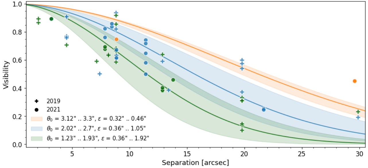
Fig. 10. Observed contrast loss at 2.2\ \mu\text{m} versus off-axis separation for the ATs. The three curves indicate the typical contrast loss for different seeing and isoplanatic angle values as expected from atmospheric turbulence following Elhalkouj et al. (2008) . Crosses represent data from GRAVITY Wide observations with the prototype implementation in November 2019, while circles represent data from GRAVITY Wide commissioning in December 2021. Seeing and isoplanatic angle values are measured by the MASS-DIMM at the Paranal observatory, and are defined at 500\ \text{nm} .
