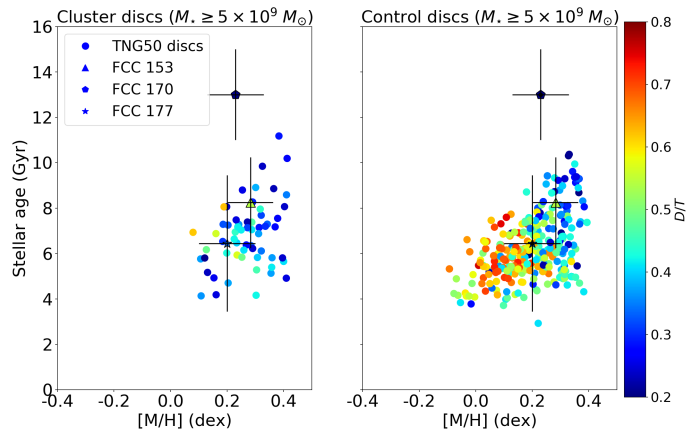
Figure 7. Mass-weighted stellar age vs metallicity near the equatorial plane for galaxies with z = 0 values of D/T \geq 0.2 and M_* \geq 5 \times 10^9 M_\odot within TNG50 Fornax-like clusters (left panel color points) and for their field counterpart matched in stellar mass (right panel color points), compared to corresponding values of the three Fornax edge-on discs FCC 153, FCC 170, and FCC 177 (triangles). Disc-over-total fraction for the three Fornax edge-on galaxies come from Ding et al. in prep and are on average 40% for FCC 153 and FCC 170 and around 15% for FCC 170. Here, stellar population properties of observed galaxies come from full spectral fitting, whereas directly from the simulation particle properties for TNG50 galaxies. Stellar discs as old and metal rich as observed in FCC 170 cannot be found in the TNG50 simulation.
