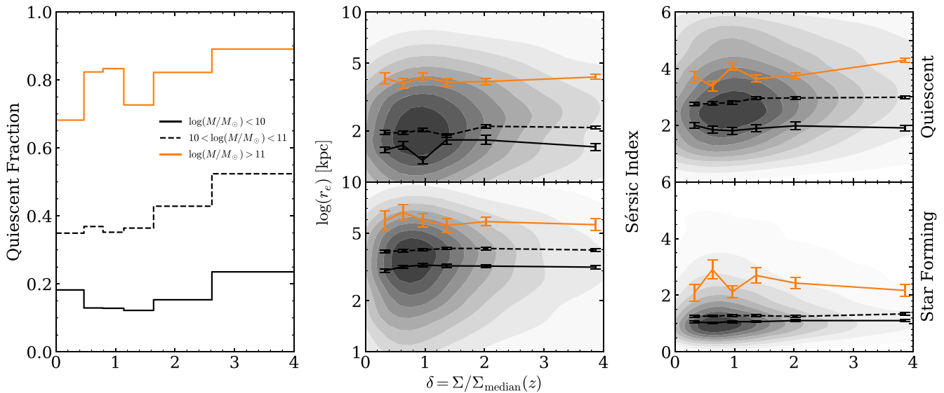
Figure 15. The constant evolution of low- ( \log(M/M_\odot) < 10 ), intermediate- ( 10 < \log(M/M_\odot) < 11 ), and high- ( \log(M/M_\odot) > 11 ) mass galaxy properties with density suggests environmental effects are not a dominant mechanism behind the flattening of the quiescent size-mass relation. The three mass regimes are represented with solid black, dashed black, and solid orange lines, respectively. The left panel shows the change in quiescent fraction for each mass bin. The other panels show the change in size (middle column) and Sérsic index (right column) for both quiescent (top row) and star-forming galaxies (bottom row). The total distributions of quiescent and star-forming sizes and Sérsic indices are shown with shaded contours.
