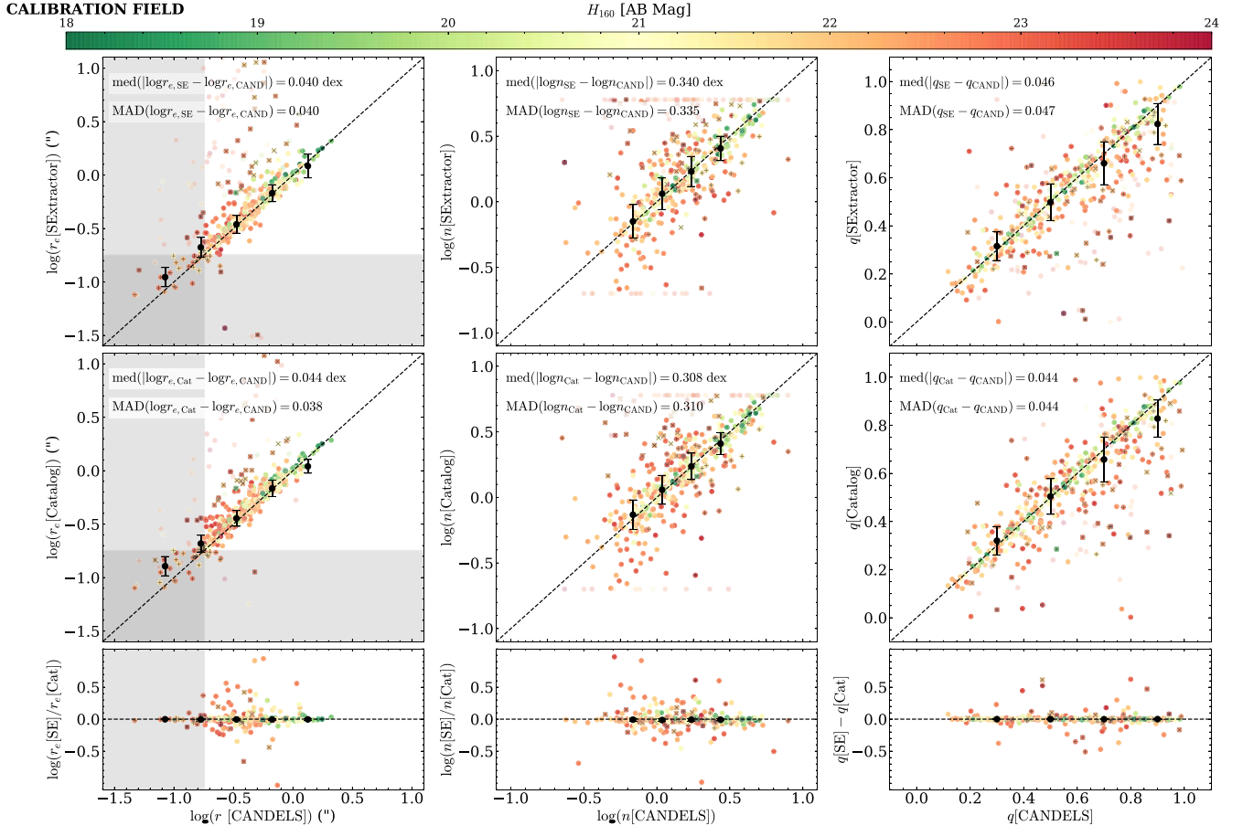
Figure 6. Scatter in the best-fit Sérsic parameters obtained using a deep-detection (Catalog) segmentation map is slightly smaller than with a DASH-depth (SExtractor) segmentation map. The top and middle rows show the effective radii, Sérsic indices, and axis ratios of the best-fit Sérsic models determined with the DASH-depth segmentation map (top) and with the catalog segmentation map (middle), respectively, compared to those from CANDELS/3DHST (van der Wel et al. 2012). Transparent points are those with flag=2 parameter values (see Section 3.1). The bottom row shows the difference in the parameters when measured both with and without fitting background. The large black points are the running median in each bin, with errorbars showing the scatter determined by the median absolute deviation (MAD) of the bin. The color scale indicates the H_{160} magnitude of the source in AB magnitudes. Points with a black x are those that are greater than 0.3 dex from the one-to-one line in radius. The gray shaded region shows radii less than the PSF FWHM and points with a black + are sources whose best-fit radius falls in this region. The median and MAD of the offset between parameters derived with the two segmentation maps and CANDELS is shown in the each panel of the top and middle row.
