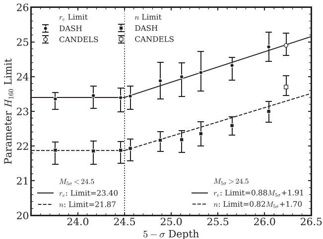
Figure 10. Magnitude limit-depth relation for effective radius and Sérsic index used in generating parameter robustness flags in the COSMOS-DASH morphological catalog. The GALFIT H_{160} limits derived in Section 3.6 and Figure 9 are compared to the 5\sigma depths computed in Section 3.6. Effective radius limits are shown with circles and Sérsic index limits are shown with squares. Limits from COSMOS-DASH (this study) are indicated by filled points while open points indicate values derived from the CANDELS/3D-HST morphological catalog (van der Wel et al. 2014). The expression describing the relation between the parameter limits and the magnitude depths is a piecewise function that is constant for depths < 24.5 and linear for depths > 24.5. The dotted line indicates a 5\sigma depth of 24.5, illustrating the two regimes of the relation. The resulting best-fit constant and linear relations are shown in the bottom left and right of the figure and the curves are indicated with a solid line for radius and a dashed line for Sérsic index.
