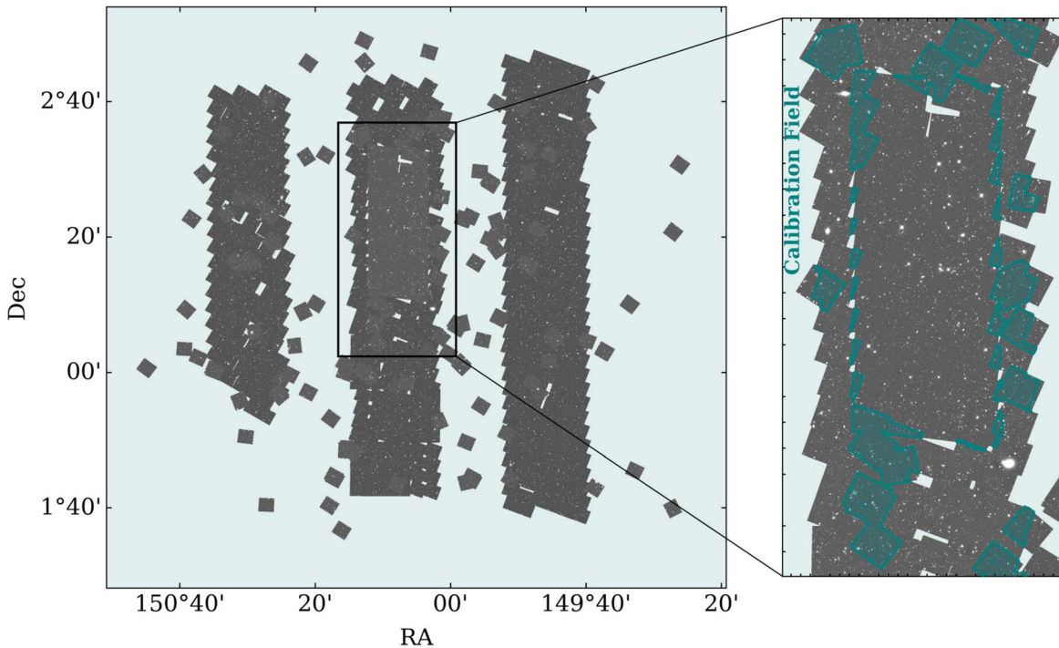
Figure 1. Image of the COSMOS-DASH mosaic, which roughly covers the UVISTA deep stripes. The left panel shows the science image of the COSMOS-DASH field with CANDELS and other archival exposures included. The inset shows the “calibration field,” which is the region of COSMOS-DASH that overlaps with CANDELS. The overlap itself is highlighted in teal, and facilitates a direct comparison of DASH and CANDELS depth morphologies.
