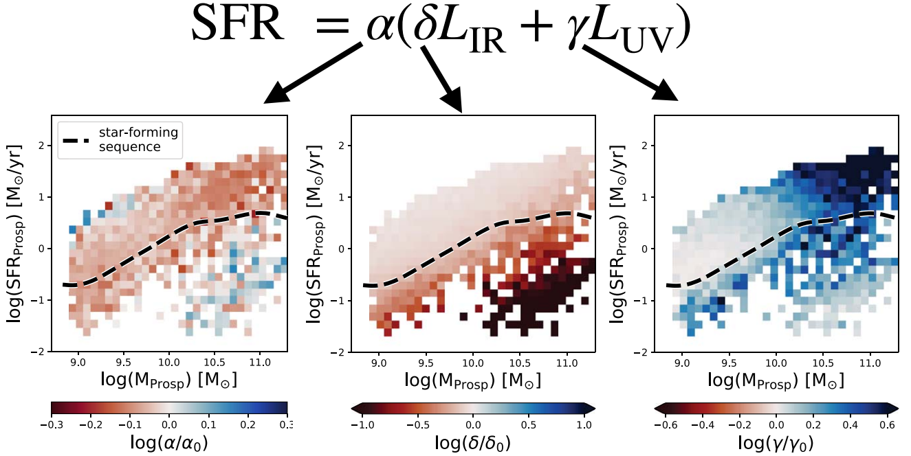
Figure 10. The median difference in the coefficients to the UV+IR SFR in Equation (11) between Prospector-α model and the fixed template-based coefficients from Bell et al. (2005) is shown for galaxies at 0.7 < z < 1.3 . \alpha parameterizes the total energy output of young stars, \delta parameterizes the fraction of IR luminosity which is powered by energy from young stars, and \gamma parameterizes the conversion from the observed UV luminosity to the bolometric luminosity of the young stars after dust attenuation. Arrows on the color bar indicate where the data is clipped to enhance the information content of the map. The y-axis shows the SFR averaged over the most recent 100 Myr.
