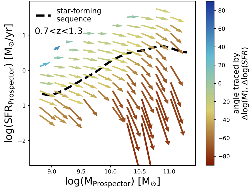
Figure 9. The median shift in inferred values of \log M^* and \log \text{SFR} between the Prospector-α model and FAST stellar masses/UV+IR SFRs for galaxies at 0.7 < z < 1.3 . Only cells with N > 20 galaxies are shown. The masses increase by \sim 0.2 dex due to the use of nonparametric star formation histories. The inferred SFRs decrease by 0.1\text{--}1+ dex largely due to dust heating from old stars, though other effects can contribute substantially in certain regimes (see Section 6.2 for an in-depth discussion). The ridgeline of the star-forming sequence as measured in this work is shown as a black dashed line. The color bar traces the angle of the shift in \log M\text{--}\log \text{SFR} space, where \theta = 0 is a horizontal arrow pointing to the right.
