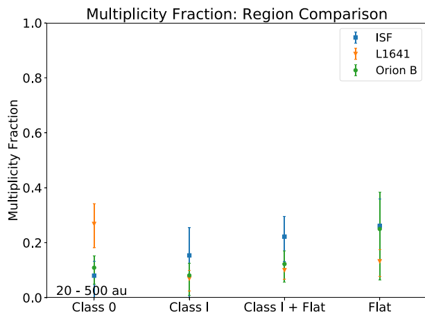
Figure 20. MFs and CFs on different scales as a function of protostar class for different regions within Orion. The MFs and CFs of the non-Class 0 protostars in the ISF are systematically higher than the other regions for separations 20 to 10^4 au, but the differences are not statistically significant.
