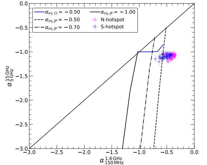
(d) Per-pixel colour-colour plot of the hotspot data of Fig. 3. We see that the emission in hotspots is inconsistent with all three ageing models.
