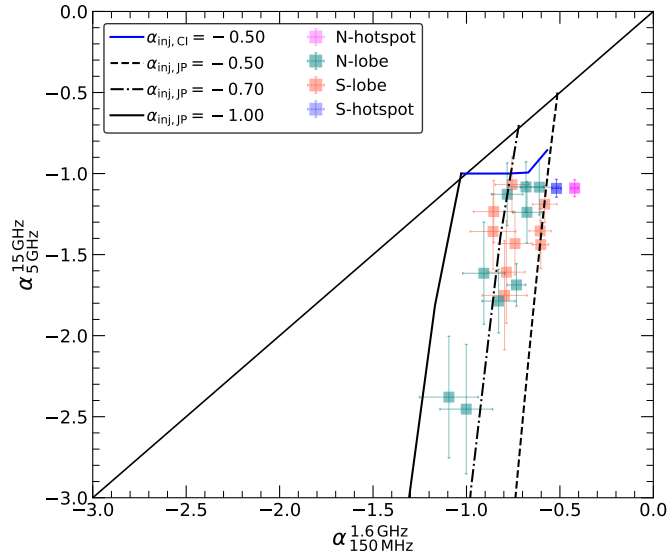
(a) Radio colour-colour plot of 3C295 overlaid with the JP and CI spectral aging models with different injection indices. The regions used for extracting the spectral indices are shown in Fig. 4b. The two North lobe outliers correspond to regions near the host galaxy.
