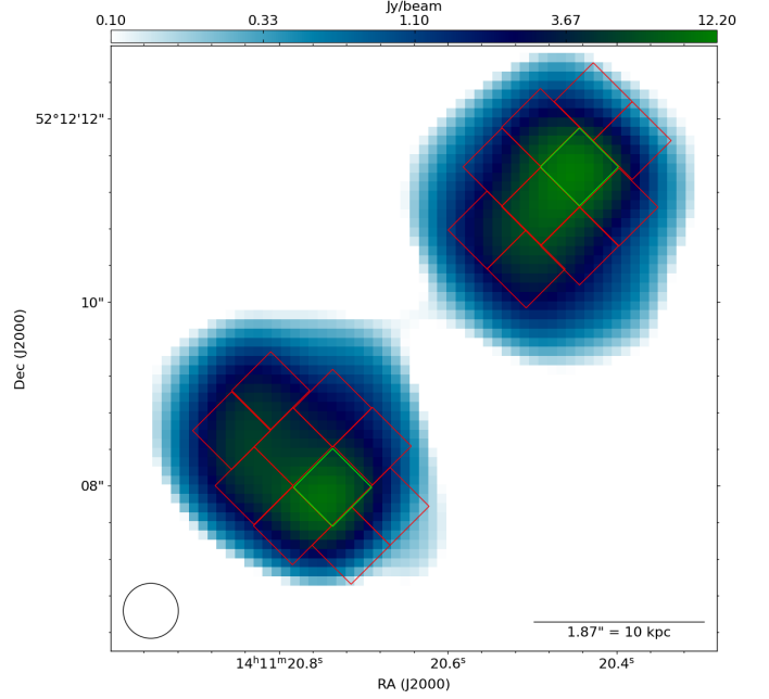
(b) Map of the regions used to calculate the colour-colour plot. Red regions are the lobe regions, and green the hotspots.
