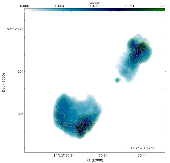
Fig. A.1: VLA map of 3C295 at 8.561 GHz, courtesy of M. Hardcastle. Pixel size is 0.05'' , beam size is 0.175'' , and flux is in Jy. The image is overlaid on itself in yellow contours starting from 0.5\sigma and going to 0.9 of the maximum flux present. 3C295 is clearly well-resolved and shows complex structure with both compact and diffuse emission present.
