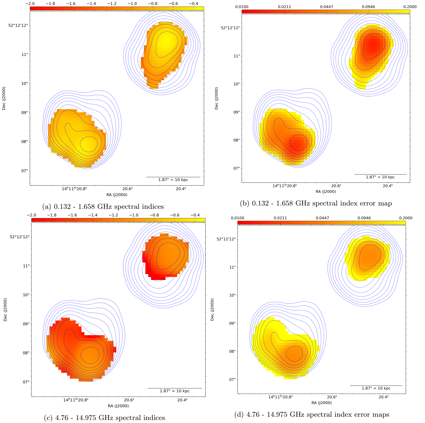
Fig. 3: Spectral index maps with associated error maps.
