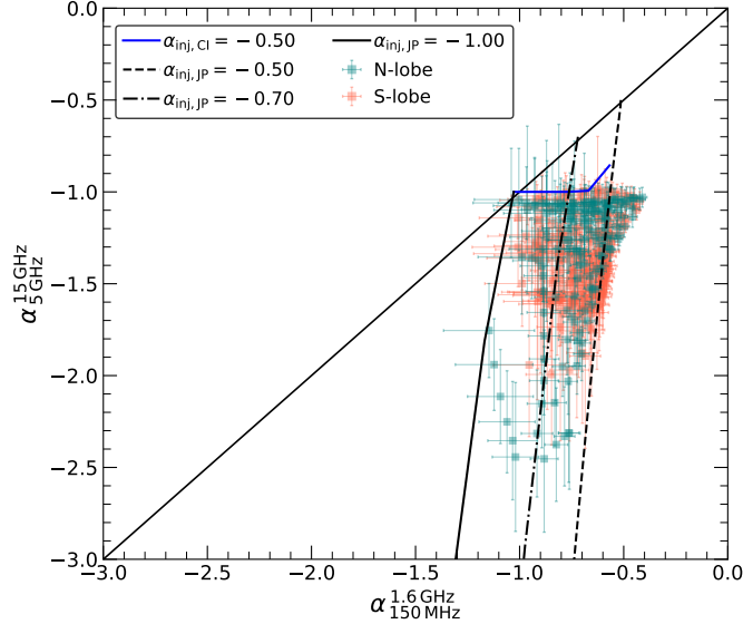
(c) Per-pixel colour-colour map to the lobes of Fig. 3. We see that the emission is largely consistent with the JP model. Outliers are pixels which are near the hotspots, and therefore likely to be contaminated by hotspot regions.
