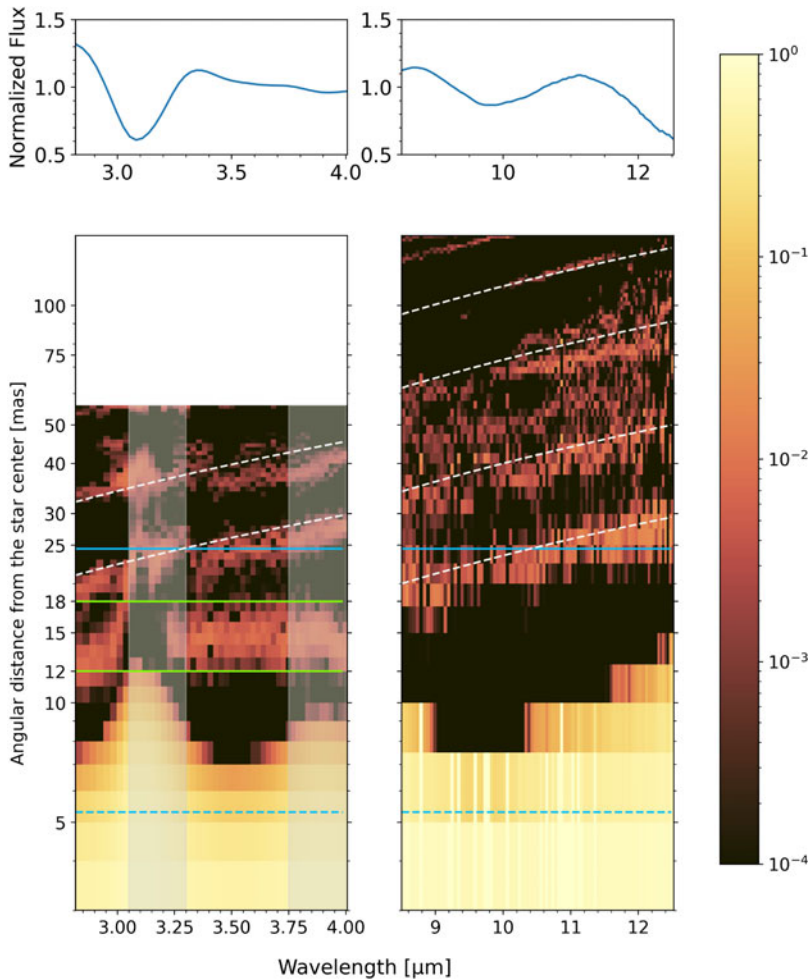
Figure 2. Upper panels correspond to the observed MATISSE spectrum normalized by the median and then divided by a black body spectra at T=2700 K to underline the observed emission and absorption features. Lower panels are the spectro-radial maps in L - and N -band obtained by plotting the best intensity Hankel profile normalized at one for each observed wavelength. The faint red structures highlighted with the inclined dashed-white lines are reconstruction artifacts. The dashed and solid blue horizontal lines show the position of the Rosseland radius and the DUSTY inner radius respectively. The solid green horizontal lines delimit the extension of a hot distinct molecular layer. The grey vertical bands cover the spectral ranges where the centro-symmetric Hankel profile is not able to properly reproduce the asymmetric shape of R Scl revealed by non-zero closure phases.
