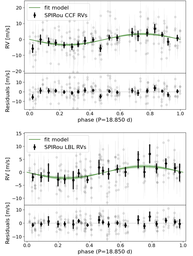
Fig. 18. TOI-1759 b orbit fit. The points in light gray show the SPIRou CCF (upper panel) and LBL (lower panel) RVs phase-folded to an orbital period of 18.850 days. Black points show weighted averages within a bin size of 0.05 ( \sim 0.95 days). The green lines and shaded regions show the best-fit models and their uncertainties for the orbit of TOI-1759 b. The residuals are displayed at the bottom of each panel, giving an RMS of 7.7 \text{ m s}^{-1} and 4.6 \text{ m s}^{-1} for CCF and LBL, respectively.
