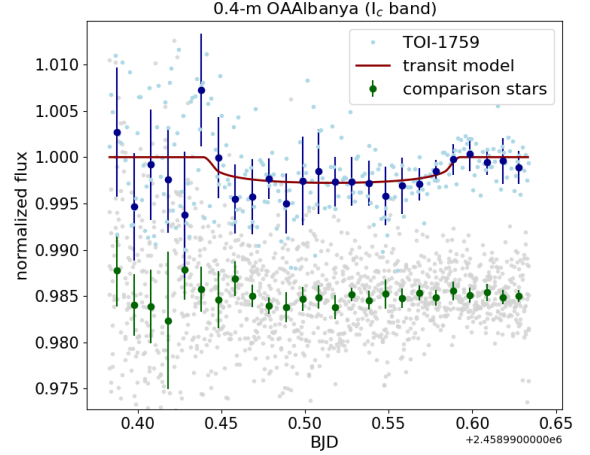
Fig. 2. Ground-based I_c -band differential photometry time series of a transit of TOI-1759 b obtained by the 0.4 m OAAlbanya observatory on May 20, 2020. The light blue points show relative fluxes of TOI-1759, and the dark blue points show weighted average bins with bin sizes of 0.01 days. The gray and green points show the relative fluxes for the comparison stars that we used in the differential photometry. The red line shows the best-fit transit model obtained from our analysis of the TESS data alone, as presented in Sect. 5.
