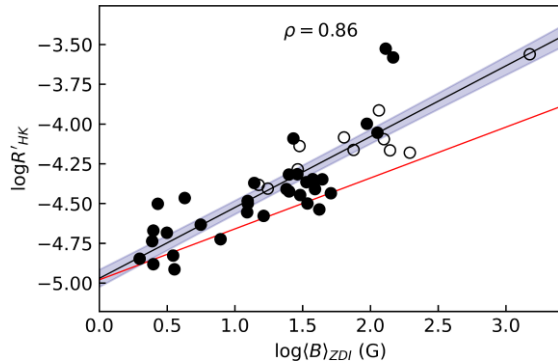
Figure 7. Mean chromospheric activity from our study versus surface-averaged large-scale magnetic field strength from published ZDI work. Marker fill-styles are the same as in Fig. 1; open circles represent young stars with strong spectral Li I lines and filled circles are mature stars assumed to be on the main sequence. The black regression line has a slope of 0.44 \pm 0.04 , and the grey shaded region shows its 95 per cent confidence interval. The red line shows the previous results of Petit et al. (2008).
