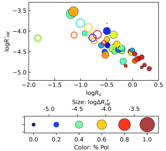
Figure D1. Mean \log R'_{\text{HK}} versus the theoretical Rossby number taken from See et al. (2019a), where marker colour shows the fractional poloidal field and marker size scales with chromospheric activity variability.
