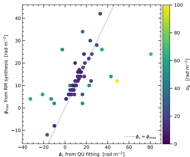
Fig. 11. Central Faraday depth, \phi_c , position of the single component from QU-fitting (see Fig. 10 brown markers, note we use here the one component fit for all boxes) versus peak position, \phi_{\max} in the RM-synthesis spectra. The color indicates the Faraday depth width of the QU-fitting component. Evidently, QU-fitting and RM-synthesis gives similar results in case of a low Faraday dispersion. Larger differences between QU-fitting and RM-synthesis correspond to higher Faraday dispersions.
