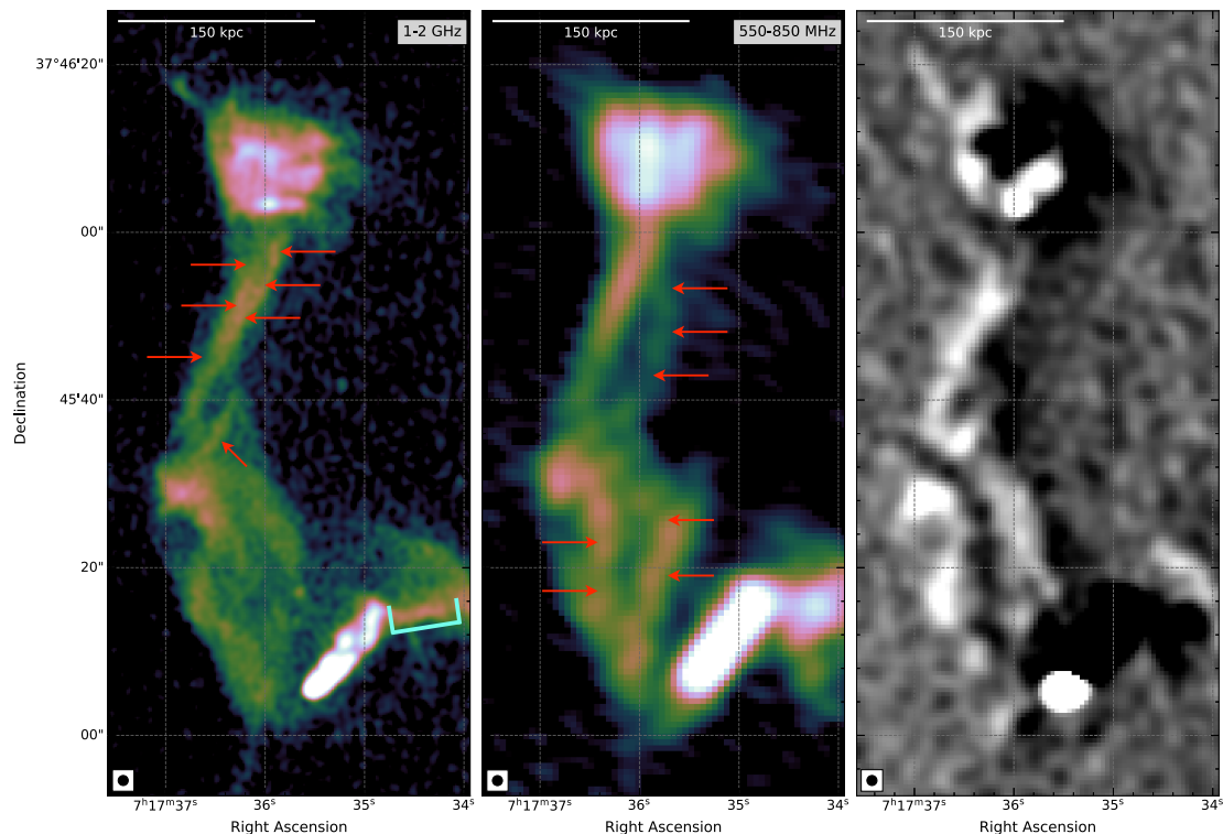
Fig. 15. High resolution VLA (left panel; van Weeren et al. 2017b) and uGMRT (middle panel; Rajpurohit et al. 2020a) images of the northern part of the relic. The red arrows show regions with fine filaments. The spectral tomography map of the same region is shown in the right panel, indicating that the relic is indeed composed of filaments with different spectral indices (Rajpurohit et al. 2021c). For the majority of these regions, the QU-fitting provides a better fit with two Faraday components.
