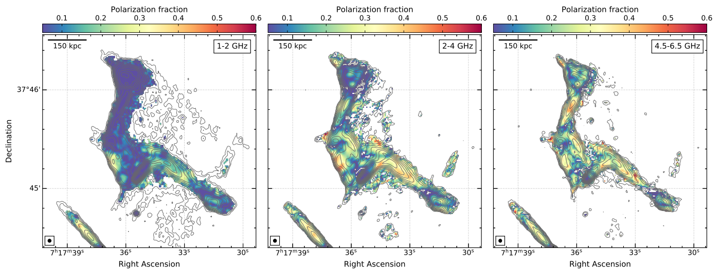
Fig. 3. High resolution ( 2'' ) fractional polarization maps at VLA L-, S-, and C-band. The relic is polarized at all of the observed frequencies, reaching values up to 50% in some regions. The northern part of the relic strongly depolarizes at 1.5 GHz. Contour levels are drawn at \sqrt{[1, 2, 4, 8, \dots]} \times 5\sigma_{\text{rms}} and are from the S-band Stokes I image. These maps are corrected for the Rician bias. The beam sizes are indicated in the bottom left corner of the each image. The image properties are given in Table 1, IM1, IM5, and IM9.
