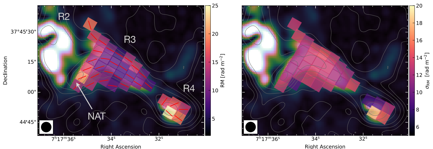
Fig. 12. \phi_c and \sigma_\phi values across the R3 and R4 region of the relic obtained with QU-fitting. For almost all boxes the one Gaussian component model is preferred, except for the region where the NAT galaxy is located. We note that for the NAT region only the low dispersion component is shown in the figure, matching the \phi_c of the relic. Moreover the left panel (red lines) shows the intrinsic polarization angle. The QU-fitting results are overlaid on the polarization intensity at 5'' and contours of the VLA L-band Stokes I image, see Table 1, IM6, for image properties. Contour levels are drawn at [1, 2, 4, 8, \dots] \times 5 \sigma_{\text{rms}} . From these maps it is evident that \phi_c and \sigma_\phi are low in this region of the relic, in particular in the R3 region, and not changing significantly from box to box. The central Faraday depth of the Gaussian components are very close to the Galactic foreground RM, indicating very little Faraday rotation due material intervening the line-of-sight to cluster outside of the Milky Way. This suggests that this part of the relic is located at the periphery of the cluster towards the observer.
