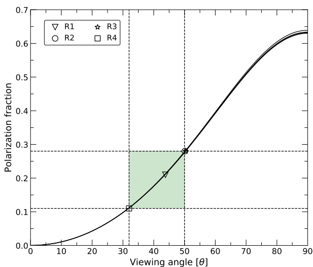
Fig. 17. Viewing angle versus polarization fraction relation for the MACS J0717.5+3745 relic. A viewing angle of 90° implies that the merger is in the plane of the sky (i.e., perpendicular to the shock). The four solid curves, that are nearly identical, give the theoretical predictions for spectral indices of \alpha = -1.18, -1.13, -1.17, and -1.16 , for the relic subregions. The triangle, circle, star, and square provide the corresponding estimates for the relic subregions R1, R2, R3, and R4. The dashed lines indicate the minimum and maximum value of the mean polarization fraction and the viewing angle. The possible viewing angles of MACS J0717.5+3745 fall inside the green shaded region. The plot shows that the relic in MACS J0717.5+3745 is seen less edge-on.
