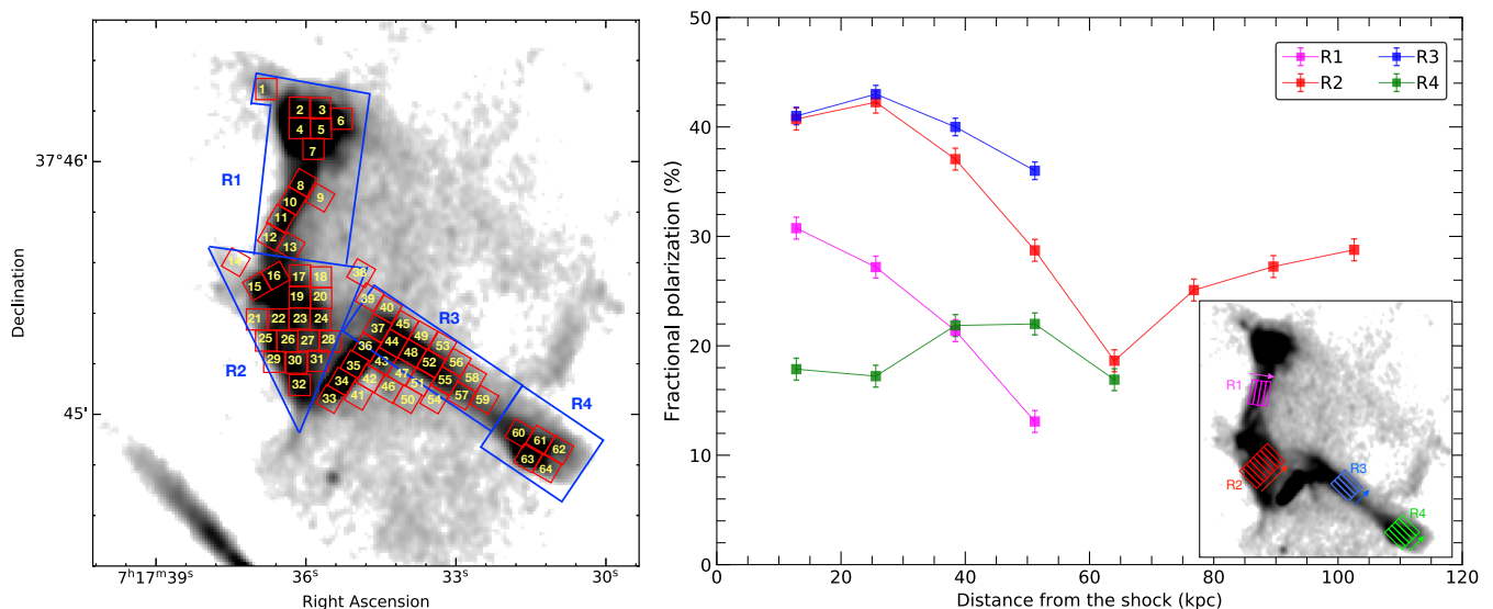
Fig. 4. Left: VLA L-band image, blue regions show the relic subregions where the average fractional polarization was extracted. The fractional polarization at R3 in Table 2 is obtained by excluding the contribution from the NAT. Red boxes where flux densities and Faraday dispersion functions were extracted for QU-fitting and RM-synthesis, respectively. Each red box has a width of 5'' , corresponding to a physical size of 32 kpc. Right: The fractional polarization profiles across the relic extracted from the rectangular regions, depicted in the inset, of width 2'' . There is a hint that the fractional polarization decreases in the downstream regions (i.e., shown with arrows).
