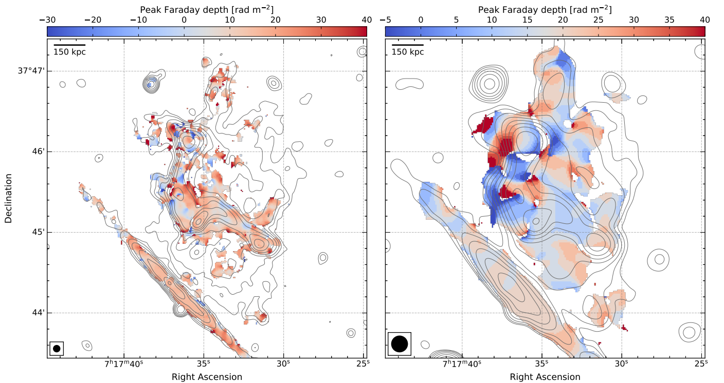
Fig. 7. Faraday depth ( \phi_{\text{max}} ) maps of the relic in MACS J0717.5+3745 measured over 1.0-6.5 GHz using RM-synthesis technique. Left: High-resolution (4'') Faraday map. The \phi_{\text{max}} distribution across the relic, in particular in the northern part is patchy with coherence lengths of 10-50 kpc. Right: Low-resolution (12.5'') Faraday depth map. The measured \phi_{\text{max}} values in the polarized halo region are similar to the R3 region of the relic, indicating very little Faraday Rotation intervening material. This suggests that these regions are located on the near side of the cluster.
