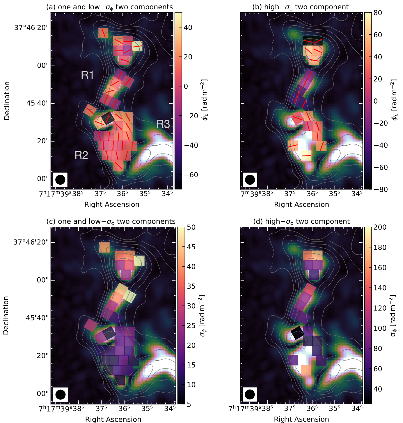
Fig. 13. Central Faraday depth and Faraday dispersion values for the northern part of the relic obtained with QU-fitting. Top: The \phi_c values for one component and low Faraday dispersion components (panel a) and the high Faraday dispersion two components (panel b). For a large number of regions, we find the presence of two Faraday components; the one component or the low Faraday dispersion component in case of two components (left panels) and the high Faraday dispersion components (right panels). Bottom: The \sigma_\phi values for one component and low Faraday dispersion components (panel c) and the high Faraday dispersion two components (panel d). The majority of the polarized emission is at rather high \sigma_\phi , suggesting that the northern part of the relic is located in or behind the ICM. Contours and image properties are as in Fig. 12.
