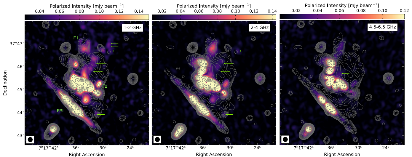
Fig. 19. Low resolution ( 12.5'' resolution) polarization intensity overlaid with the total intensity contours, showing that a part of the halo is polarized (shown with green arrows). Contour levels are drawn at \sqrt{[1, 2, 4, 8, \dots]} \times 4 \sigma_{\text{rms}} and are from the S-band Stokes I image. The beam sizes are indicated in the bottom left corner of the image. The image properties are given in Table 1, IM4, IM8, and IM12.
