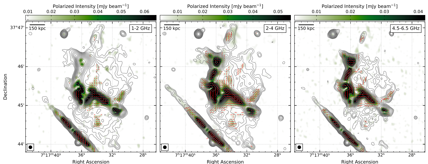
Fig. 5. Polarization intensity maps ( 5'' resolution) at VLA L-, S-, and C-band after performing RM-synthesis. Red lines represent the magnetic field vectors. Their orientation represents the projected B-field corrected for Faraday rotation and contribution from the Galactic foreground. The vector lengths are proportional to the polarization percentage and their lengths are corrected for Ricean bias. No vectors were drawn for pixels below 5\sigma in the polarized intensity image. The distinct filaments, namely F1 and F2 (for labeling see Fig. 1), and some regions embedded in the halo emission are polarized between 10–38% between 1 and 6.5 GHz. At all the observed frequencies, the B-field across the relic and other features is highly-ordered. Contour levels are drawn at \sqrt{[1, 2, 4, 8, \dots]} \times 5\sigma_{\text{rms}} and are from the VLA L-band, S-band and C-band Stokes I images at 1.5 GHz, 3 GHz and 5.5 GHz, respectively. The image properties are given in Table 1, IM2, IM6, and IM10. The beam sizes are indicated in the bottom left corner of the each image.
