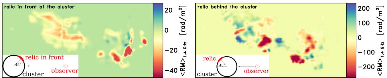
Fig. 18. Simulations: maps of the average RM, radio weighted at 1.4 GHz. Left: the RM distribution if the relic lies in front of the cluster, as depicted in the inset. Right: the RM distribution if the relic lies behind the cluster, as show in the inset. These maps show that strong fluctuations in the RM are expected if the relic is located within, or behind, the ICM screen.
