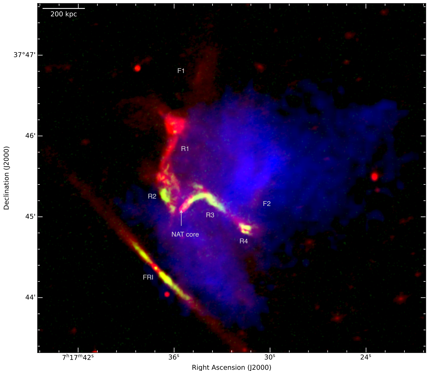
Fig. 1. Composite total power, polarization intensity, and X-ray image of the relic in MACS J0717+3745 at 2'' resolution. The total power and L-band polarization emission are shown in red and green-yellow, respectively. The intensity in blue shows the X-ray emission. The lack of polarized emission in the north region (R1) indicates depolarization. The image properties are given in Table 1, IM5 and IM9.
