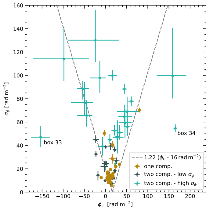
Fig. 14. Central Faraday depth as a function of Faraday dispersion, measured in the observers frame. Dashed-lines indicate \sigma_\phi = 1.22(\phi_c - 16 \text{ rad m}^{-2}) where 16 \text{ rad m}^{-2} is the Faraday depth due to the Galactic foreground. One component models are indicated with brown filled circles and two component models with black and cyan stars, where black indicates the component with the lower Faraday dispersion and cyan the higher one. Components shown in Fig. 10 with a very large uncertainties are neglected here because they do not provide any constraint. The plot shows that the scatter of the central Faraday depth increases with increasing Faraday dispersion.
