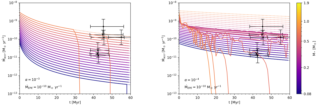
Figure 3. The accretion rates as a function of time for all discs that live to at least 50 Myr under an EPE rate of 10^{-10} M_\odot \text{ yr}^{-1} , for a viscosity parameter of \alpha = 10^{-3} (left) and \alpha = 10^{-4} (right). The dotted lines are the prescribed accretion rates, and the solid lines are the actual accretion rates. The colour indicates host star mass, with dark purple corresponding to 0.08 M_\odot . Note that the accretion rate is a monotonically increasing function of host star mass. Also shown are the observed ages and accretion rates of the Peter Pan discs listed in Silverberg et al. (2020) and Lee et al. (2020) as black points with error bars (the latter did not provide error estimates, so we opted to conservatively display the largest error bars of the sample of Silverberg et al. (2020) ). The two clusters of three points have the same ages, but we have displaced them horizontally for visibility. The left-most point of the clusters corresponds to their true age.
