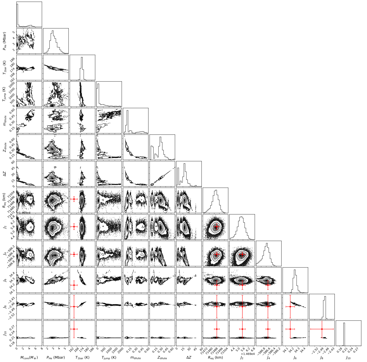
Fig. A.6: Resulting distributions obtained with the dilute-core model and MLS20 equation of state.
