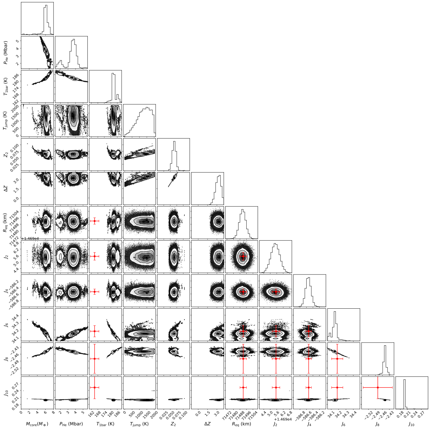
Fig. A.1: MCMC corner plot showing the posterior distribution of variables obtained with the 3-layer model and the MH13 equation of state. Red points with error bars show the observed parameters as a reference.
