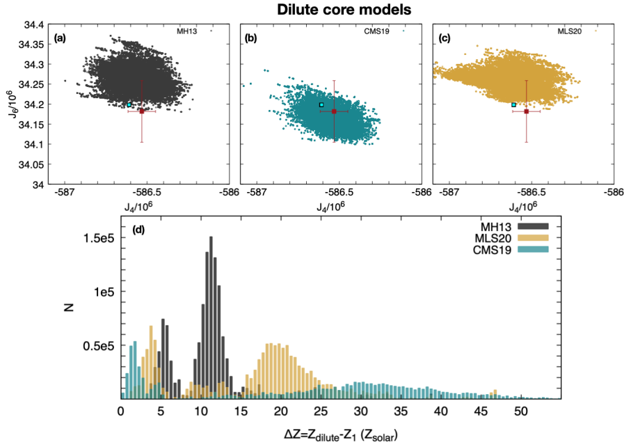
Fig. 6: Specifics of models with dilute core. Panels (a), (b) and (c): J_4 vs. J_6 obtained considering different equations of state for H. The Juno measurement ( J_{2n}^{\text{Juno}} ) is indicated with the cyan square. The effective gravity harmonics to be matched by our interior models ( J_{2n}^{\text{static}} ) are shown in red. Panel (d): Histogram that shows the difference in heavy elements ( \Delta Z = Z_{\text{dilute}} - Z_1 ) between the dilute core region and the H_2 -dominated layer.
