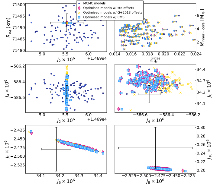
Fig. 3: Results for 4 sets of 100 models : random models from our preferred MCMC runs, optimised models with new offsets, optimised models with former offsets from Guillot et al. (2018) and optimised models with CMS calculation. Top left panel : Equatorial radius vs J_2 . Top right panel : Core mass vs fraction of ices in the molecular hydrogen layer. Grey lines show the pairing between each model and its optimised version. Middle and bottom panels : Gravitational moments. The black error bars show the uncertainty of the Juno measurements accounting for the differential rotation.
