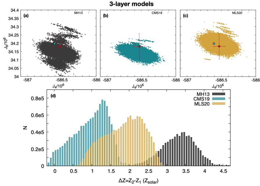
Fig. 5: Details of models with 3 layers. Panels (a), (b) and (c): J_4 vs. J_6 for 3-layer models calculated using different equations of state for H, indicated in the Figure. Cyan squares show the Juno measurements ( J_{2n}^{\text{Juno}} ), and gravitational harmonics corrected by differential rotation –the ones to match with our interior models ( J_{2n}^{\text{static}} )– are shown in red. Panel (d): Histogram showing the difference in heavy elements ( \Delta Z = Z_2 - Z_1 ) between the H_{\text{metallic}} - and the H_2 -dominated layers.
