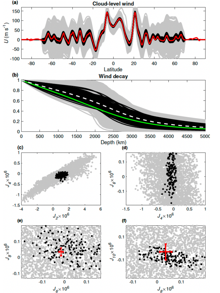
Fig. 4: Contribution to the gravity harmonics from the deep atmospheric flow. Shown are the solutions for the cloud-level wind (a), the radial decay profile (b), and the wind-induced even gravity harmonics (c-f). The grey lines/dots show all of the 3000 cases, and the black lines/dots show the plausible solutions. The red line in (a) shows the observed cloud-level wind, and the green line in (b) shows the solution in Kaspi et al. (2018). The red crosses in (e-f) show the expected mean value of the differential contribution.
