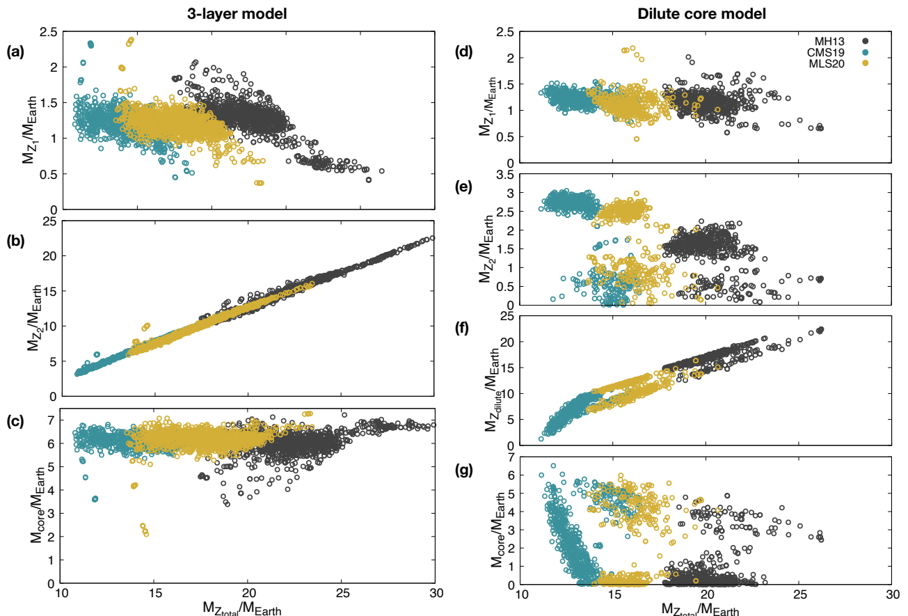
Fig. 7: Mass of heavy elements in the different layers as a function of the total mass of heavy elements in Jupiter for a random sample of 1000 models extracted from our 3 layer models (a, b and c) and from models with a dilute core (d, e, f, and g). Different colours show models calculated with different equations of state. Panels (a) and (d) show the mass in the \text{H}_2 -dominated region in the y-axis, panels (b) and (e) show the mass in the \text{H}_{\text{metallic}} -dominated region, panel (f) shows the mass in the dilute core and panels (c) and (g) show the mass in the inner core.
