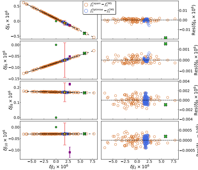
Fig. 2: Offsets between ToF and CMS for two subsamples (MCMC models & optimised models). Left panels : Offsets on the gravitational moments. The black dashed line shows the linear fit of our models. The green dot shows the origin. The yellow star corresponds to the linear fit of the optimised models median of \Delta J_2 . The pink error-bars shows the uncertainty of the Juno measurements accounting for the differential rotation. The purple error-bars show the uncertainty of the Juno measurements. The green cross shows the former offsets from Guillot et al. (2018). Right panels : Residuals.
