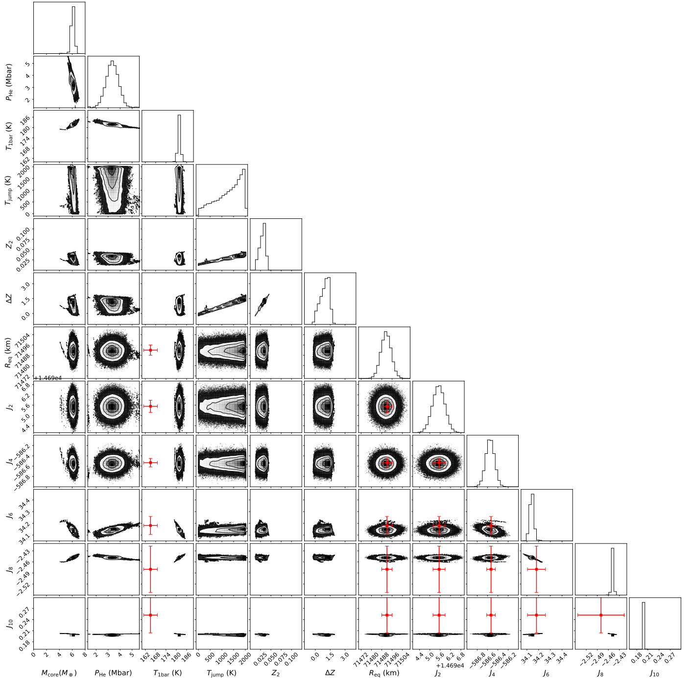
Fig. A.2: Posterior distribution resulting of the MCMC runs with 3-layers and CMS19 equation of state. Observed parameters are indicated with the red points.
