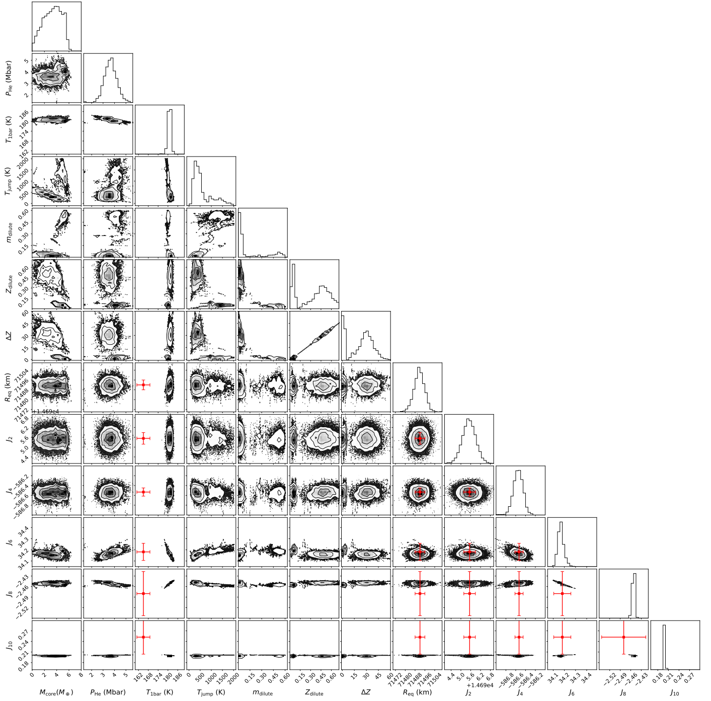
Fig. A.5: Distribution of different parameters resulting from the runs with the dilute-core model and CMS19 equation of state.
