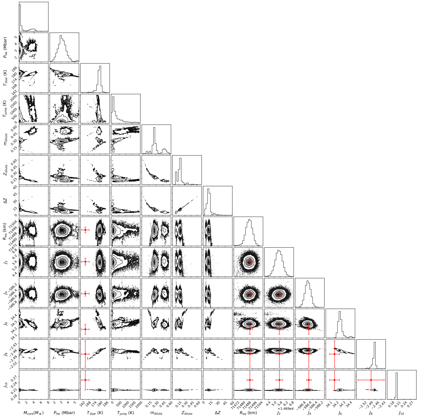
Fig. A.4: Corner plot resulting from the runs with the dilute-core model and MH13 equation of state. Red dots show observed parameters.
