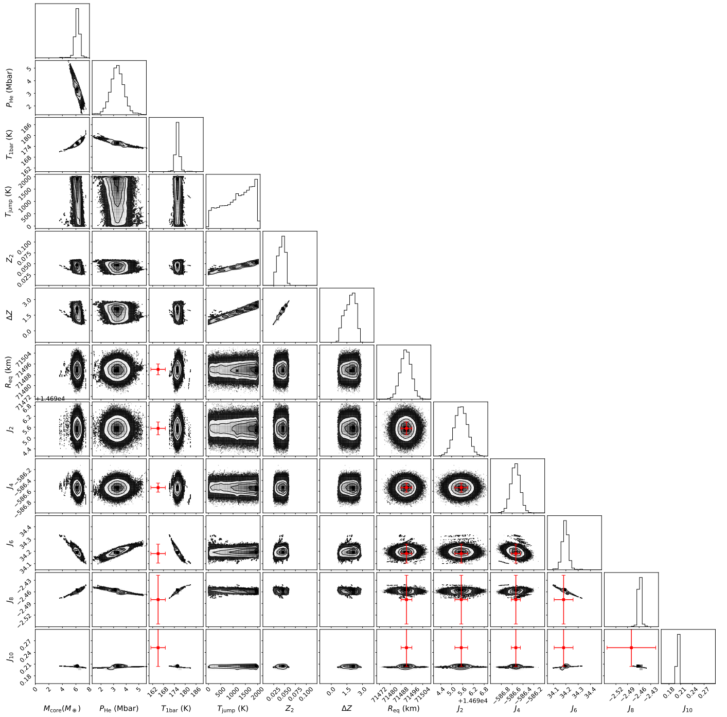
Fig. A.3: Distributions resulting of the MCMC runs with 3-layers and MLS20 equation of state.
