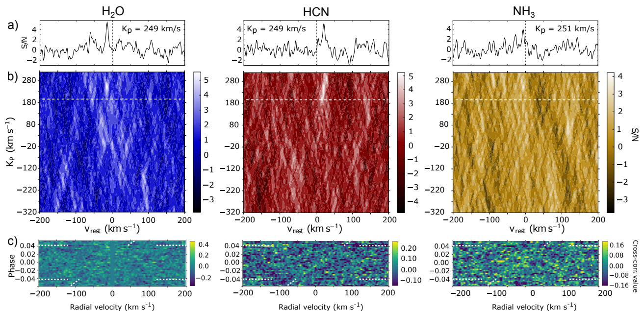
Fig. 2. Results of the cross-correlation analyses. (a) CCFs at the K_p presenting the maximum significance peak. (b) Cross-correlation maps (expressed as S/N) of potential signals for H 2 O (left), HCN (middle), and NH 3 (right) with respect to the exoplanet rest-frame velocity (horizontal axis) and K_p (vertical axis). The horizontal dashed lines mark the expected K_p of WASP-76 b ( \sim 196 km s -1 ). (c) Cross-correlation matrices in the Earth rest-frame. The transit occurs between the horizontal dashed lines and the tilted dashed lines mark the velocities of the highest significance signal. Larger versions of the cross-correlation matrices in the Earth’s rest frame and in the rest-frame of the exoplanet are shown in Appendix B.
