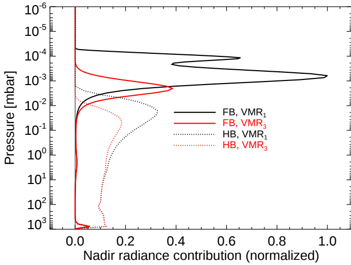
Fig. 6. Contributions to the upward radiance of the fundamental v_3 (FB, solid) and hot v_3+v_4 (HB, dashed) bands of \text{CH}_4 at the different pressure levels for the \text{VMR}_1 (black) and \text{VMR}_3 (red) profiles. The p - T_1 profile and the nominal non-LTE collisional rates of Table 1 were used in all cases. All values have been normalised to the maximum of the v_3 band for \text{VMR}_1 .
