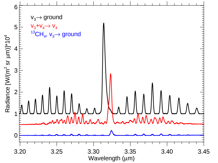
Fig. 5. Contributions of CH 4 bands to the ISO nadir radiances near 3.3 μm for the p-T 1 temperature, the CH 4 VMR 1 profile, and the nominal collisional rates (see Table 1). A vertical offset of 0.5 units was included between the different radiances for clarity.
