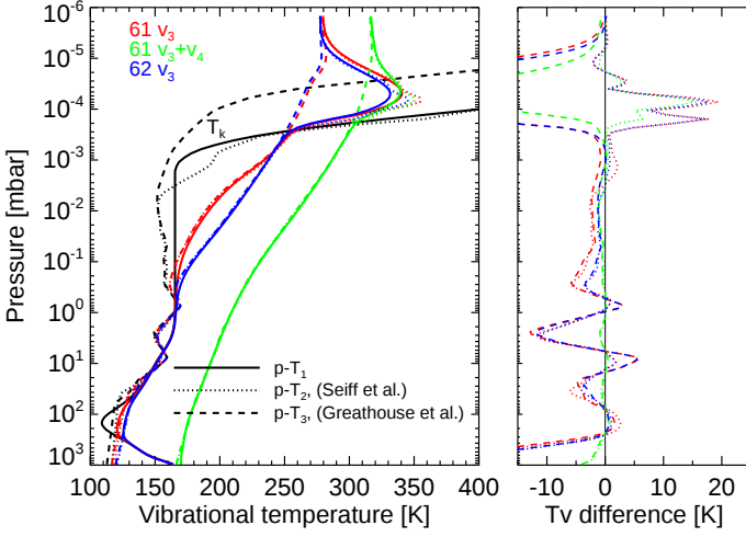
Fig. 9. Effects of the kinetic temperature profiles p-T 1 , p-T 2 , and p-T 3 on the CH 4 vibrational temperatures for the main energy levels that contribute to the ISO 3.3 \mu m radiance. The VMR 1 profile and the nominal collisional rates were used.
