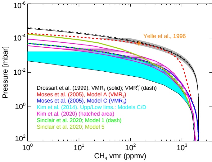
Fig. 3. CH 4 volume mixing ratio profiles considered in this work. The black dashed profile (VMR 1 R ) is the CH 4 abundance that we derived in our analyses. The grey shaded area are the errors obtained by propagating the uncertainties of the collisional rates, temperature, and calibration error (see Sect. 5). The rest of the curves correspond to different profiles available in the literature, as labelled in the figure.
