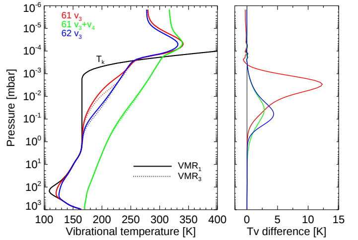
Fig. 7. Effects of the \text{CH}_4 \text{VMR} on the \text{CH}_4 vibrational temperatures for the main energy levels that contribute to the ISO 3.3 \mu\text{m} radiance. The p - T_1 kinetic temperature profile and the nominal collisional rates were used.
