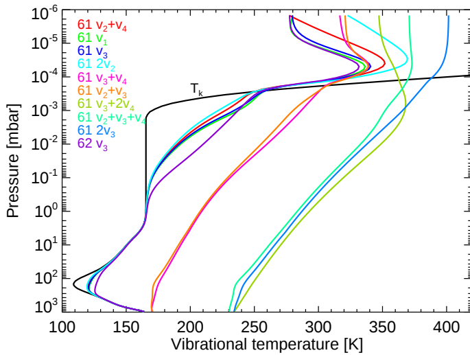
Fig. 2. Daytime (SZA=0°) vibrational temperatures of the main CH 4 energy levels contributing to the 3.3 μm radiance as a function of pressure. The p-T 1 kinetic temperature profile, the VMR 1 abundance profile, and the nominal collisional rates of Table 1 were used. The major CH 4 isotopologue is labelled ‘61’ and the second is labelled ‘62’.
