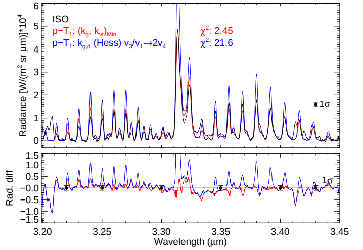
Fig. 15. Measured (black) and synthetic (red and blue) spectra. The red spectrum assumed the p-T 1 and VMR 1 R profiles and the k_{g,Min} and k_{vt,Min} rates. The blue spectrum is obtained assuming the collisional rate k_{g,d} instead of k_{g,c} (see Table 1) and also including the relaxation of v_1 by the same process. The 1 \sigma noise error of the measurements is also shown.
