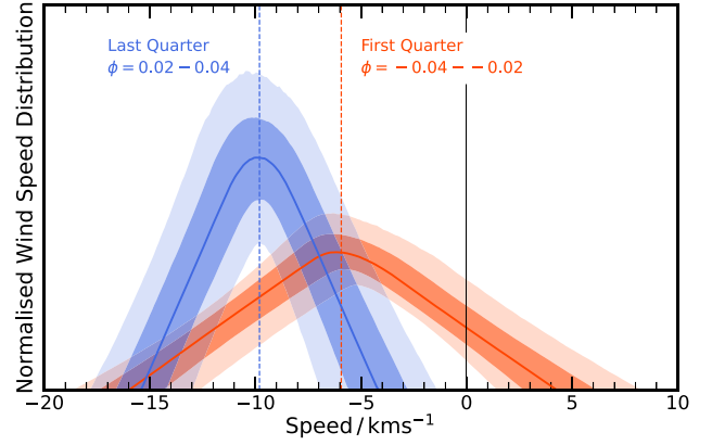
Figure 14. Normalized wind speed distribution as derived from the \Delta V_{\text{sys}} and \delta V_{\text{wind}} parameters given in Fig. 13. This is the day–night wind broadening kernel applied to the model as shown in Fig. 2. The constraints on the \phi = -0.04 to -0.02 range are shown in red and the constraints on the \phi = 0.02 – 0.04 range in blue. The dashed lines indicate the median values of \Delta V_{\text{sys}} from our retrieval. The negative values indicate a day–to–night wind, which results in a net blueshift of the overall spectrum.
