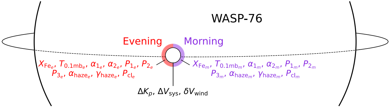
Figure 1. Schematic of the transit of WASP-76 b and the retrieval parameters for HyDRA-2D. For each of the evening and morning limbs, we retrieve the gaseous iron abundance with X_{Fe} , the temperature profile is set through the six parameters T_{mbar} , \alpha_1 , \alpha_2 , P_1 , P_2 and P_3 using the parametrization in Madhusudhan & Seager (2009), and the opacity and haze are parametrized with \alpha_{haze} , \gamma_{haze} , and P_{cl} . We also retrieve \Delta K_p , \Delta V_{sys} , and \delta V_{wind} to constrain the wind profile of the atmosphere (see Section 2.3).
