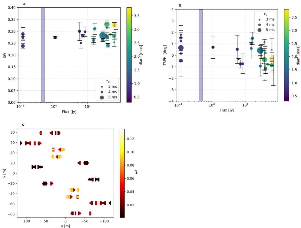
Extended Data Figure 1. MATISSE Faint Calibrator data and uv-coverage. a: Instrumental Visibility and b: non-calibrated closure phases of calibrators observed during the months of September 2018, May 2019 and June 2019, at 3.4 \mu\text{m} . Data points are colour-coded by their diameters, and the size of the circles correspond to the average coherence times, of the observations. The vertical blue strip covers the approximate correlated flux of NGC 1068 at the same wavelength.
