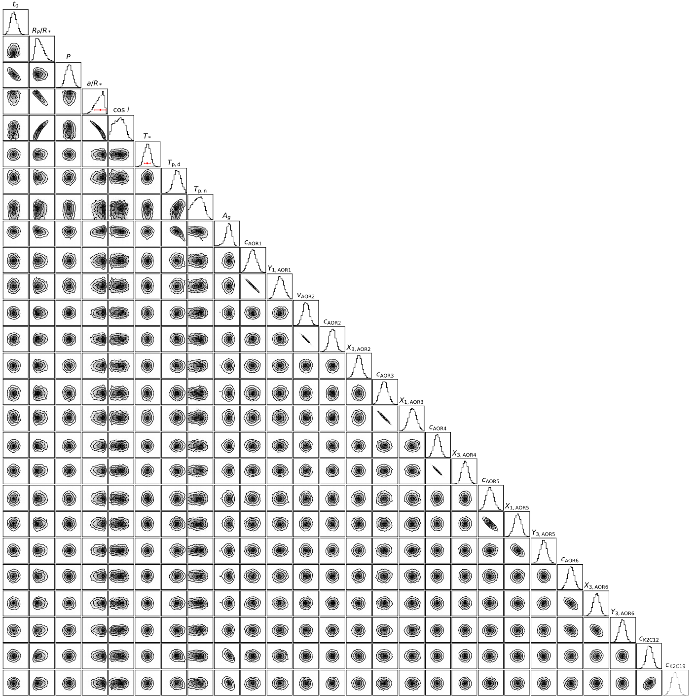
Fig. C.13: MCMC corner plot for the two temperature model fit to the joint dataset, i.e., Spitzer and K2. The red bars for a/R_* and T_* show the Gaussian priors which were used in this fit. The prior values and the best fit values are listed in Table 5. The resulting values for the systematic parameters are in Table B.4. A list with all fit parameters can be found in Table B.3.
