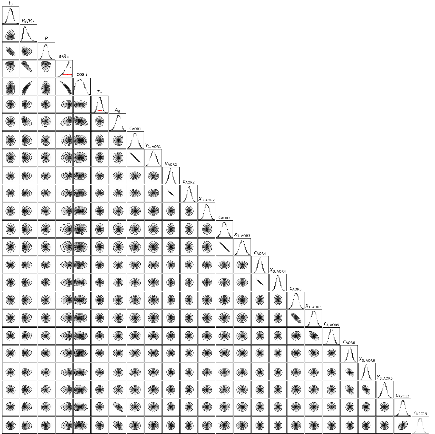
Fig. C.11: MCMC corner plot for the toy model fit without heat redistribution ( F = 0 ) to the joint dataset, i.e., Spitzer and K2. The red bars for a/R_* and T_* show the Gaussian priors which were used in this fit. The prior values and the best fit values are listed in Table 5. The resulting values for the systematic parameters are in Table B.4. A list with all fit parameters can be found in Table B.3.
