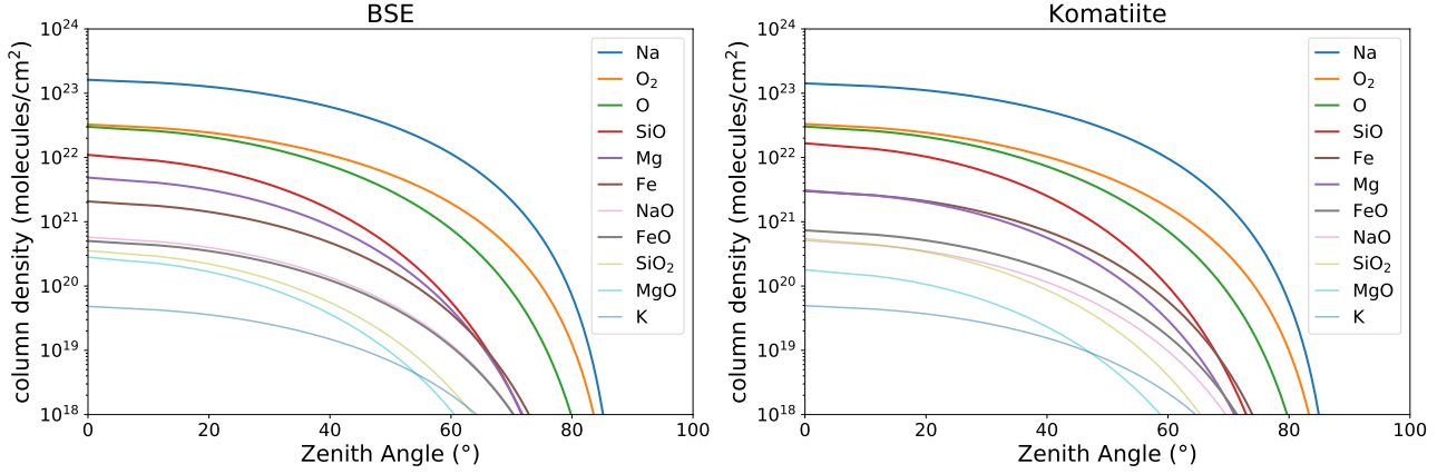
Fig. 8. Column density of various species as a function of the zenith angle of the planet for a Bulk-Silicate-Earth composition ( left panel ) and a komatiite composition ( right panel ) based on calculations in Miguel et al. (2011). The temperature as a function of zenith angle assumed for this plot is based on our best fit model presented in Kreidberg & Loeb (2016) without heat redistribution ( F = 0 ). It assumes that the temperature at the substellar point is T_{\text{substellar}} = \left(\frac{S(1-A_B)}{\sigma}\right)^{1/4} = \frac{T_{\text{eff}}}{\sqrt{a/R_*}} (1 - A_B)^{1/4} and T_{\text{terminator}} = 0 K at a zenith angle of z = 90^\circ , with S being the insolation, A_B the Bond albedo and \sigma the Stefan–Boltzmann constant. The species in the legend are sorted by the column density at the substellar point in descending order.
