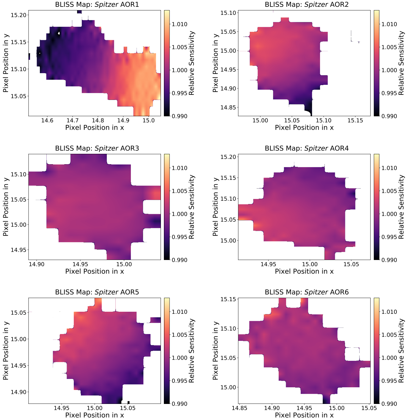
Fig. C.6: BLISS sensitivity maps for all six Spitzer AORs.
