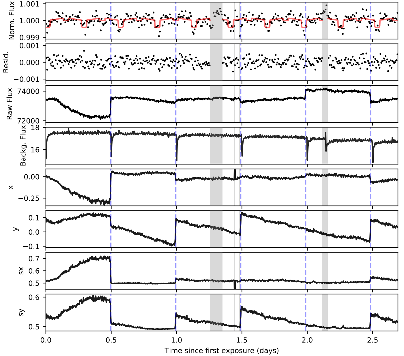
Fig. C.1: Diagnostic plot of the full Spitzer observations: The vertical, dashed blue lines indicate the start of a new Astronomical Observation Request (AOR). The data in the vertical, gray shaded regions were removed for the fit due to systematic effects. The red line in the top panel shows the best fit model of the Spitzer data. The difference between the model and the normalized flux can be seen in the panel below. The data has been binned down to 10 minutes in the top two panels and to 4 minutes in the lower panels. The observed raw flux in \mu\text{Jy}/\text{pixel} is shown in the third panel. The background flux in the fourth panel is showing changes at the beginning of every AOR as expected due to changes in pointing. An outlier segment in AOR5 which was manually removed from the dataset has been able to be attributed to a strong cosmic ray hit on the detector. The 2D images showing this event can be found in Fig. C.2. The parameters, x and y are the pixel position of the target relative to the “sweet spot”. Finally, sx and sy describe the Gaussian widths of the star’s point spread function.
