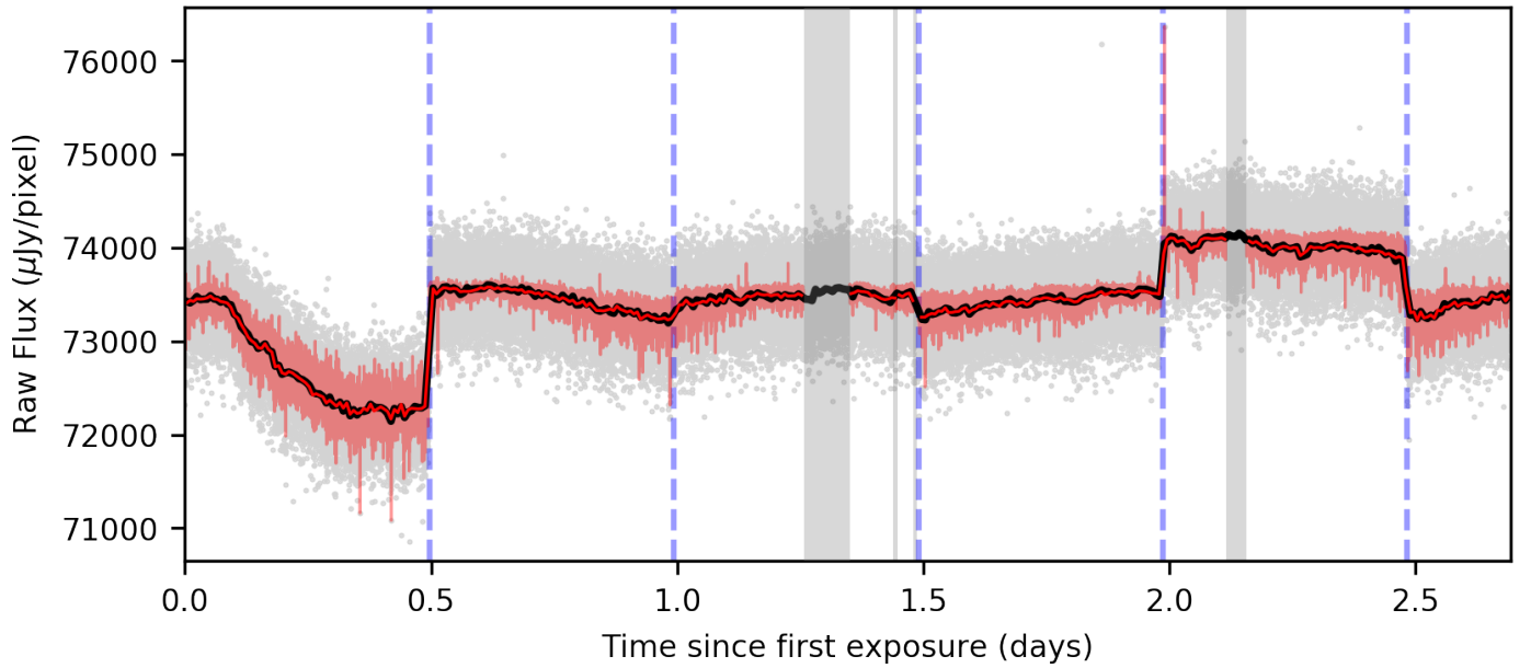
Fig. C.3: Raw, unbinned light curve is shown with gray dots with the best fitting model in light red. The vertical, dashed blue lines indicate the start of a new Astronomical Observation Request (AOR). The data in the vertical, gray shaded regions were removed for the fit due to systematic effects. The solid black (red) line shows the raw light curve (best fitting model) binned down to 10 minutes. The planetary signatures (transit, phase curve variation or eclipse) are too weak to be seen in the raw data. For example, the transit depth of K2-141 b is \sim 425 ppm which leads to a dip of just \sim 30 \mu\text{Jy/pixel} .
