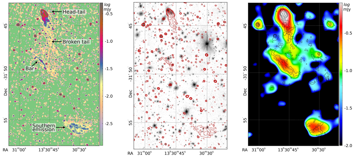
Fig. 10. 1.283 GHz MeerKAT image of the head-tail in SCJ1329–313 (left panel). The colour scale is in the range -1 - 0.1 \text{ mJy beam}^{-1} . The restoring beam of the image is 7.66'' \times 7.28'' , in p.a. 68^\circ . The various features of diffuse emission are indicated. Contours of the same image overlaid on the ESO-VST r -band image (central panel). The contour levels are \pm 20, 40, 80, 160 \mu\text{Jy beam}^{-1} . The first contour corresponds to \sim 3\sigma . Right panel - 1.283 GHz MeerKAT image of the diffuse emission at the resolution of 40'' \times 40'' in colour with GMRT contours at 306 MHz overlaid. The contours are drawn at 0.2, 0.4, 0.8 \text{ mJy beam}^{-1} . The angular resolution is 14.0'' \times 9.5'' .
