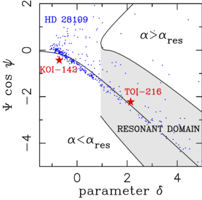
Figure 9. The 3:2 resonance structure diagram following Nesvorný & Vokrouhlický (2016). Systems with \alpha = a_c/a_d < \alpha_{\text{res}} ( \alpha > \alpha_{\text{res}} ), where \alpha = 0.763 corresponds to the exact resonance, have orbits just wide (narrow) of the resonance. The resonance region where \psi librates is shaded. The separatrices and stable point are solid. Three planetary systems are plotted: HD 28109 (this work), TOI-216 (Dawson et al. 2021; Nesvorný et al. 2021) and KOI-142 (Nesvorný et al. 2013). TOI-216 is firmly in the resonance and KOI-142 is firmly outside the resonance. For HD 28109, the blue dots show a sample of 500 posterior solutions from our dynamical 3-planet fit, of which roughly two-thirds are non-resonant and roughly one-third are resonant.
