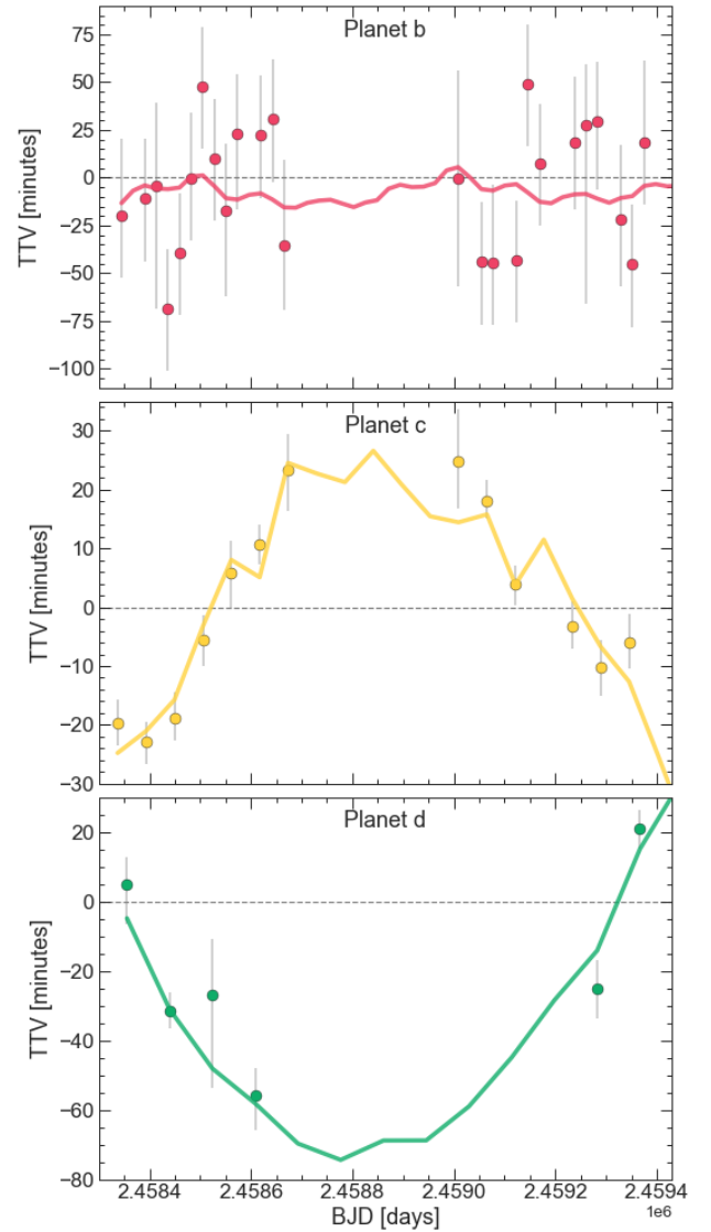
Figure 8. Transit timing variations (in minutes) for each of the planets of HD 28109 spanning two years of TESS data plus ground-based photometric monitoring of planet c. The points show the difference between the fitted mid-times and the linear predictions, while the lines show the model predictions from our dynamical analysis in Section 5.2.2.
