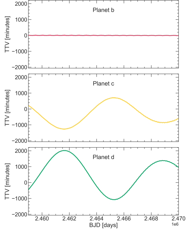
Figure 10. Model predictions of the transit timings variations for the planets of HD 28109 for the next 11 000 days, spanning more than one full TTV period for the two outer planets.
