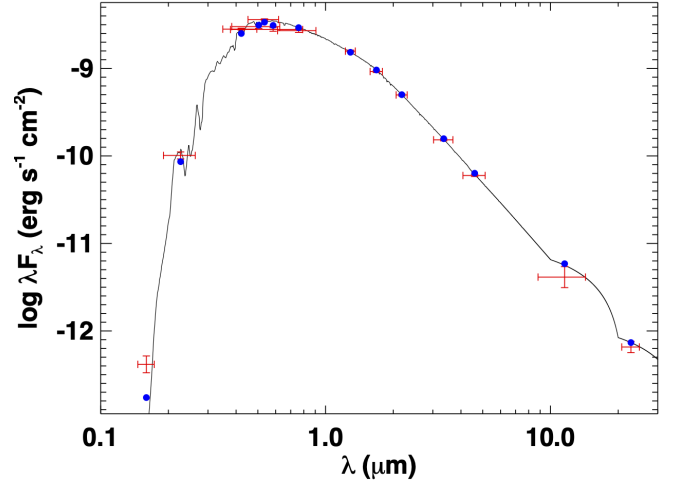
Figure 1. Spectral energy distribution (SED) of TOI-282. Red symbols represent the observed photometric measurements, where the horizontal bars represent the effective width of the passband. Blue symbols are the model fluxes from the best-fit Kurucz atmosphere model (black).
