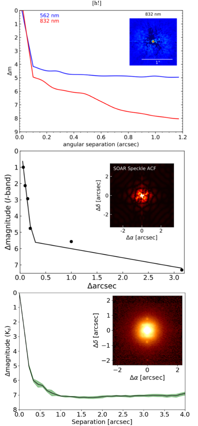
Figure 4. Contrast curves for HD 28109/TOI-282. The top panel shows the results from Gemini South, the middle panel shows the results from SOAR, and the bottom panel shows results from VLT/NaCo. All three panels are inset with final reconstructed images; none of the observations revealed bound companions within 5 magnitudes of the target.
