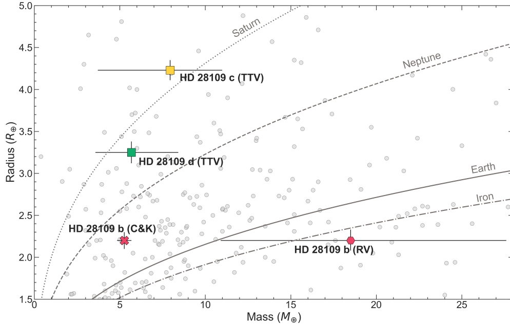
Figure 13. Mass-radius diagram showing the positions of HD 28109 b, c and d. Planets c and d are plotted as squares with their masses are estimated from TTVs. As the mass of planet b is still poorly constrained, we plot its position using its RV estimated mass as a hexagon, while the average mass for planets of its radius (estimated mass following Chen & Kipping (2017) ) is plotted as a cross.
