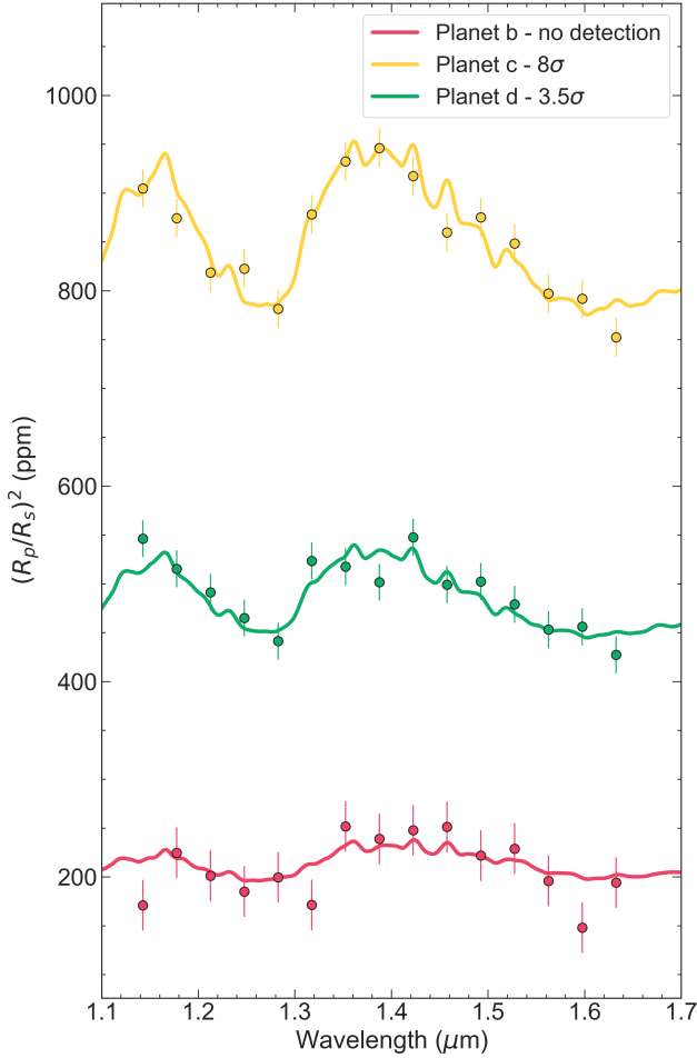
Figure 14. Model transmission spectra of HD 28109 b, c and d with simulated HST observations. Each point corresponds to a single transit depth with no offset; the curves represent the simulated transmission spectra.
