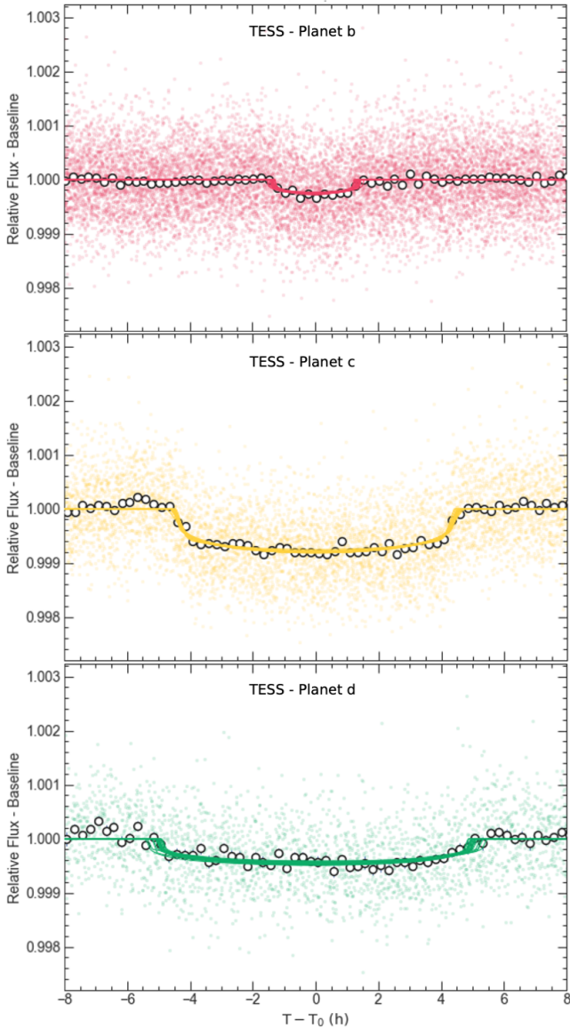
Figure 7. Global fit of the TESS photometric data for each of the planets of HD 28109. Points in the background are the phase-folded 2-minute cadence data, while white circles are the binned points. Curves are 20 samples drawn from the posterior.
