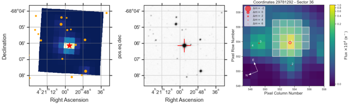
Figure 5. Images of the field of TOI-282/HD 28109, showing that the star does not have any bright contaminating sources nearby. Left Panel: Target pixel files showing TOI-282 as a red star and other nearby sources as orange circles. The size of the circles is representative of the source’s brightness. Middle Panel: Sloan Digital Sky Survey (SDSS York et al. 2000 ) image of the surrounding field of TOI-282 (indicated by a red cross). Right Panel: TESS target pixel file of one of the 25 sectors in which TOI-282 was observed, created with TPFLOTTER ( Aller et al. 2020 ). The pipeline aperture is shown by the white shaded region, and all nearby sources from Gaia ( Gaia Collaboration et al. 2018 ) down to a magnitude difference \Delta M = 8 are overplotted as red circles.
