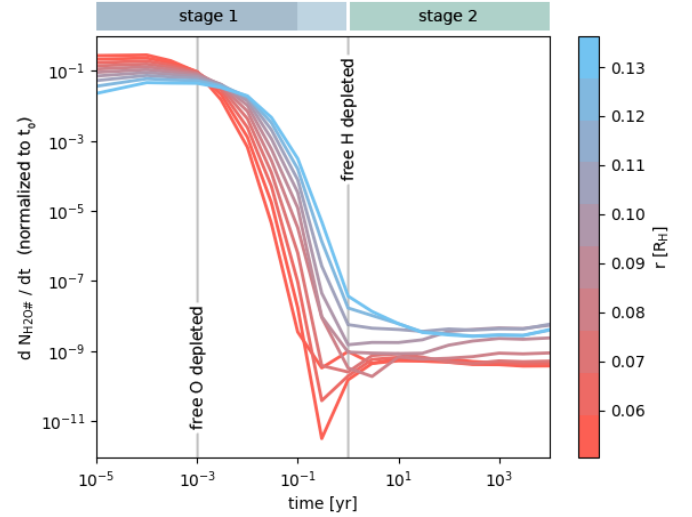
Fig. 5. Rate of water ice formation as a function of time at different radii beyond the snowline in the high-mass, high-viscosity CPD ( 7\text{--}10 ), to illustrate the two distinct stages of water ice formation. All values are normalized to the maximum formation rate at 10^{-5} \text{ yr} , r = 0.08 R_H . The times where the decline in the abundance of free O and free H end are indicated by the gray vertical lines. The starting time t_0 is defined as when the infalling gas is shock-heated to an atomic and ionized state.
