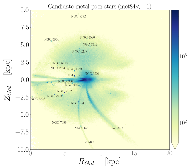
Fig. 10. Density map for bona fide candidate metal-poor stars ( \text{met}84 < -1 ; 1.58M stars) in galactocentric coordinates. Some prominent overdensities corresponding to Galactic globular clusters and the direction towards the Magellanic System are annotated.
