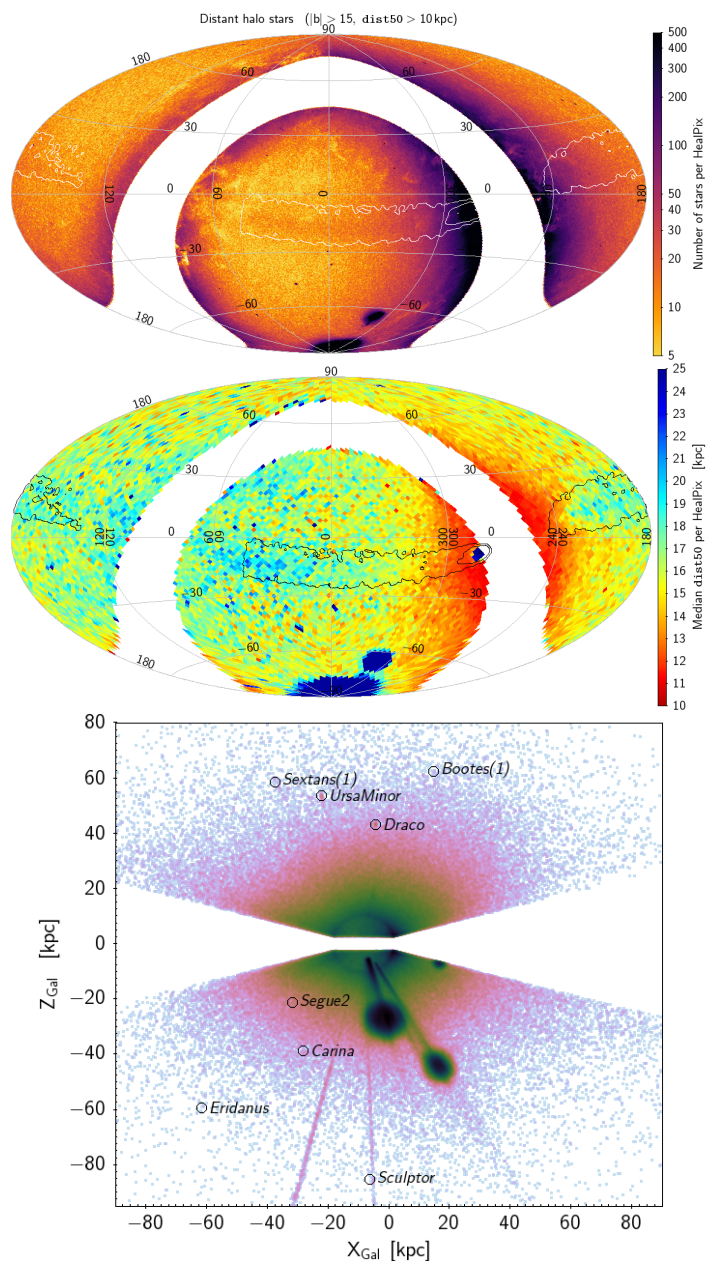
Fig. 11. Distribution of distant halo stars, selected by excluding the Galactic plane and a cut in median distance ( |b| > 15 deg, \text{dist}50 > 10 kpc; 2.55M stars). The top panel shows the sky distribution in ecliptic coordinates, highlighting the presence of the Sagittarius stream close to the ecliptic plane. The middle panel shows the same projection, colour-coded by the median distance per HealPix. In both panels the contour overlay shows the location of the Sagittarius stream candidates from Antoja et al. (2020). The bottom panel shows a Cartesian projection ( X_{\text{Gal}} vs. Z_{\text{Gal}} ), highlighting some of the less prominent Local Group objects included in the priors.
