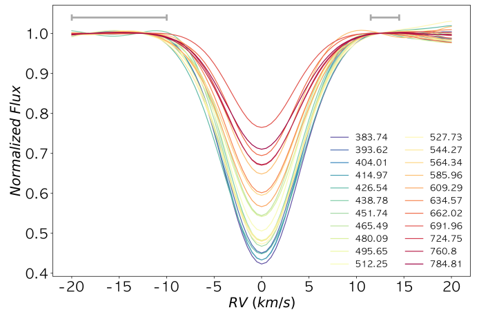
Fig. 1: Master CCF of each bin (central wavelength of each bin given in nm) from the Night 1 eight-slice-bin data sets. The solid gray lines mark the continuum regions of the CCFs that were used in the normalization.
