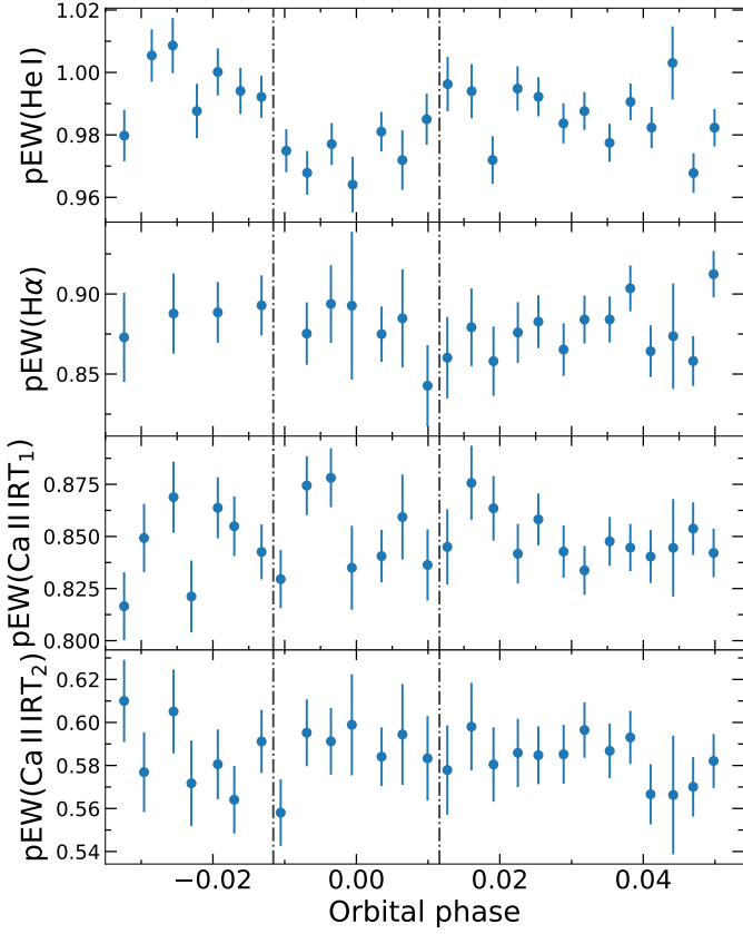
Fig. 6: Time evolution of the pseudo-equivalent widths of an He I triplet, H \alpha , and Ca II IRT \lambda 8500 Å and \lambda 8544 Å lines (from top to bottom). The vertical dashed lines mark the T1 and T4 contacts of transit of GJ 1214 b.
