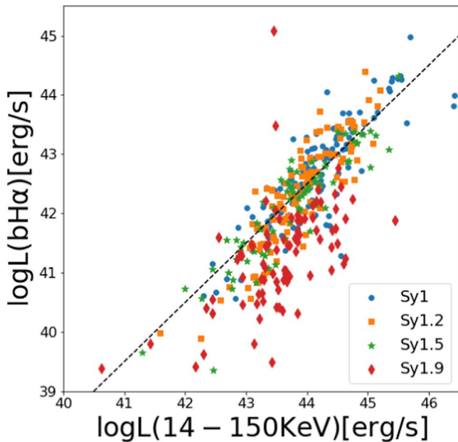
Figure 6. Broad H\alpha emission-line luminosity ( L(bH\alpha) ) vs. ultrahard X-ray luminosity ( L_{14-150\text{ keV}} ) for BASS/DR2 AGNs. Symbol colors mark AGNs of different (emission line) subclasses, as indicated in the legend. The dashed line marks a scaling of \log(L[bH\alpha])/L_{14-150\text{ keV}} = -1.5 , which describes the general trend seen in most of our bona fide broad-line AGNs. The broad H\alpha emission in Type 1.9 AGNs, however, appears suppressed relative to AGNs of other subclasses with comparable L_{14-150\text{ keV}} .
