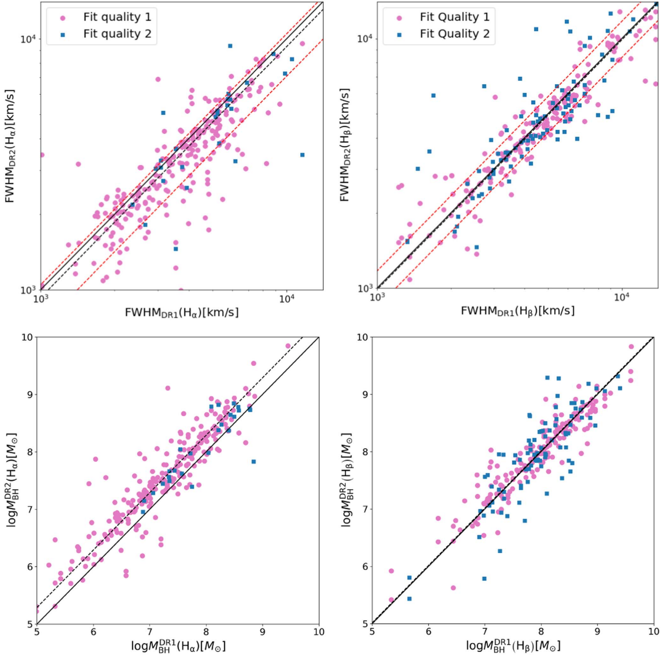
Figure 14. Comparison between DR1 and DR2 measurements: line widths (FWHM; top) and BH masses ( M_{\text{BH}} ; bottom), for both H\alpha (left) and H\beta (right). In all panels, black solid lines represent the 1:1 relation and black dashed lines trace the median offsets between DR1 and DR2 measurements.
