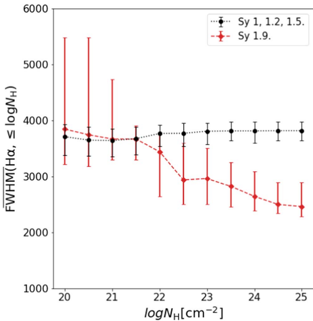
Figure 10. Median FWHM( \text{H}\alpha ) for objects with N_{\text{H}} smaller than the N_{\text{H}} in the \log N_{\text{H}} (horizontal) axis. The error bars are obtained from bootstrapping and correspond to a confidence level of 90%. Type 1.9 AGNs, which tend to have higher column densities ( \log(N_{\text{H}}/\text{cm}^{-2}) > 22 ) typically also have narrower \text{H}\alpha broad emission lines.
