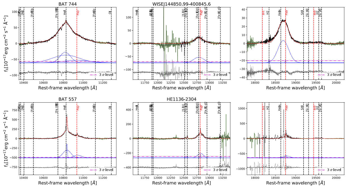
Figure 3. Examples of spectral emission-line fits of the \text{Pa}\gamma (left), \text{Pa}\beta (center), and \text{Pa}\alpha (right) regions for a Sy 1 (BAT 744, top) and a Sy 1.9 (BAT 557, bottom). The best-fit Gaussians are plotted in blue. As explained in Section 3.1, a broad Gaussian component is discarded if its intensity is below 3\sigma (dashed purple line) with respect to the fitting continuum. The continuum has been evaluated in the regions highlighted in green and subtracted off. In red the resulting total model is shown. Residuals are plotted offset in dark gray. The fit quality flags are as follows: 2, 2, and 1 in the \text{Pa}\gamma , \text{Pa}\beta , and \text{Pa}\alpha regions of BAT 744, respectively; and 2, 1, and 4 in the \text{Pa}\gamma , \text{Pa}\beta , and \text{Pa}\alpha regions of BAT 557, respectively. The complete figure set with all the 65 FIRE/Magellan spectral emission-line fits in the \text{Pa}\gamma , \text{Pa}\beta , and \text{Pa}\alpha regions is available online.
