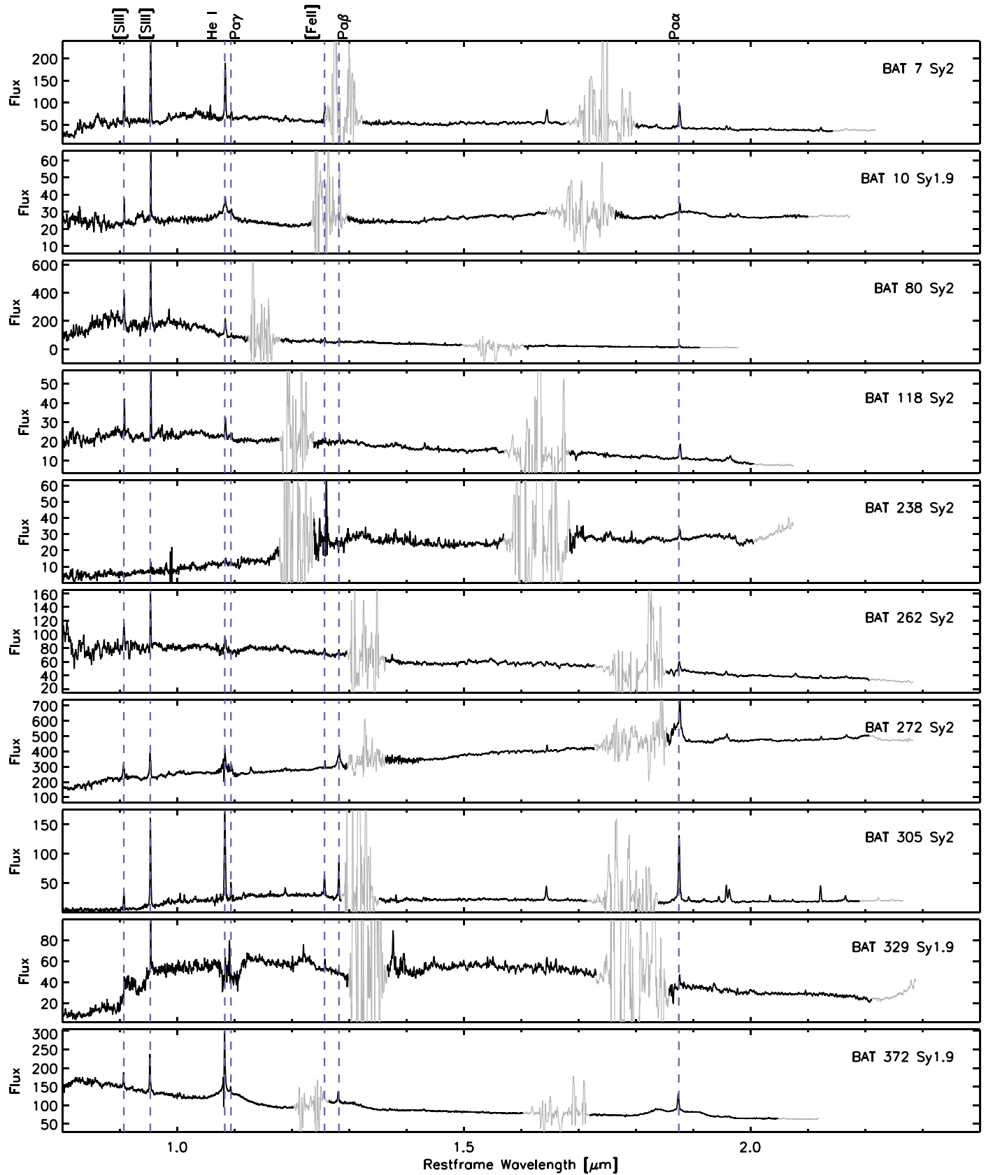
Figure 2. Examples of FIRE/Magellan NIR spectra in units of \times 10^{-17} \text{ erg s}^{-1} \text{ cm}^{-2} \text{ \AA}^{-1} , redshift-corrected and flux calibrated. The wavelength position of some of the most relevant emission lines are indicated with dashed vertical lines and labeled at the top. Regions of low telluric transmission are shown in gray. The complete figure set for the 65 AGN is available online, ordered by BAT ID.
