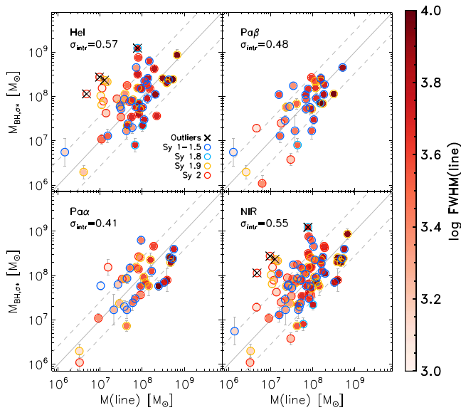
Figure 13. Comparison of M_{\text{BH},\sigma_x} vs. M(\text{line}) in BASS Sy AGN color-coded according to the \text{FWHM}(\text{line}) . The 1:1 relation is shown in solid gray, with dashed gray lines indicating the intrinsic spread. The measurements are evenly distributed around the one-to-one relation, with a clear gradient in \text{FWHM}(\text{line}) : objects with faster BLR velocities are preferentially below the unity locus, while smaller FWHMs are mostly located above the 1:1 relation, in all the lines examined.
