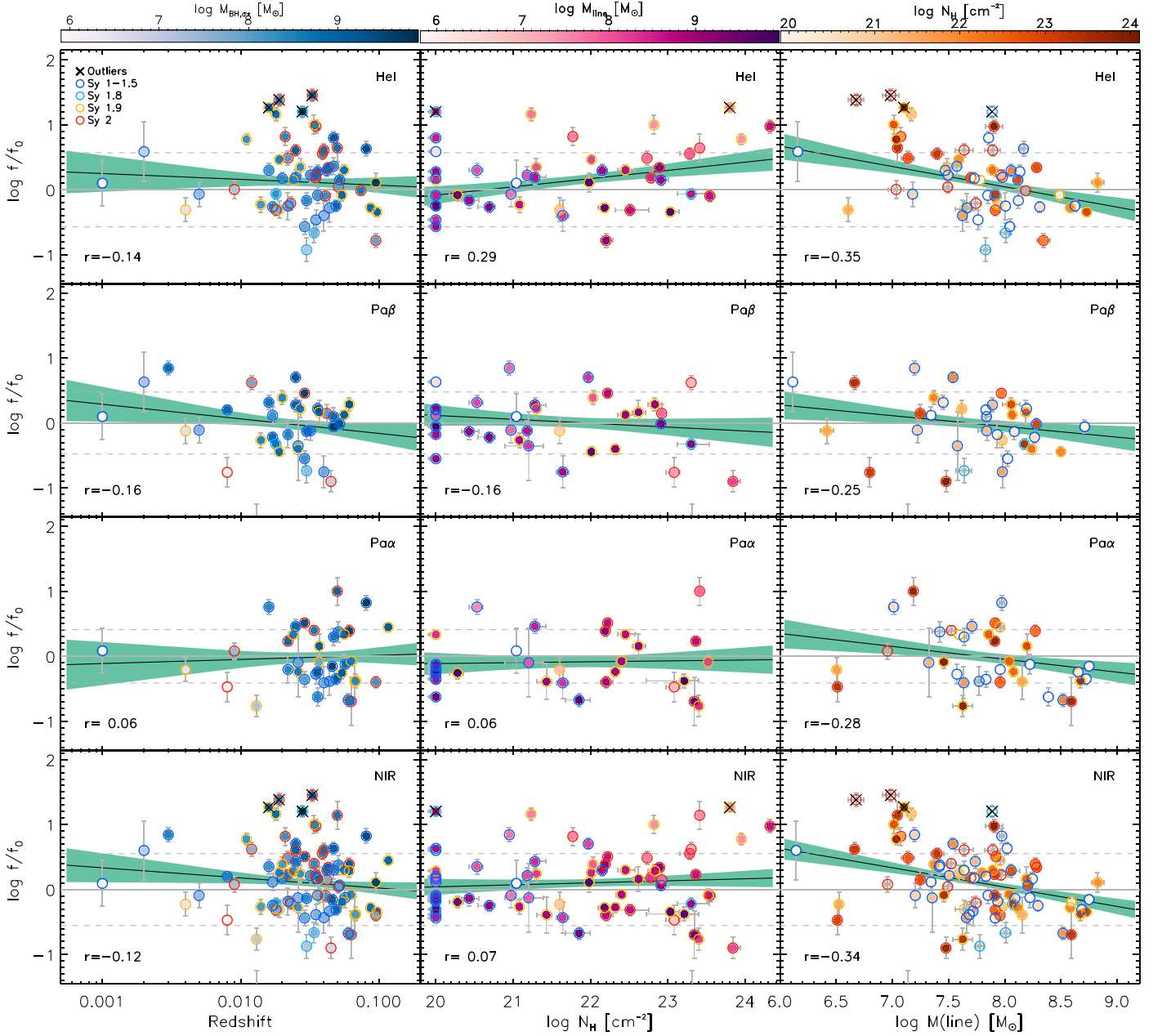
Figure 14. Comparison between the offset M_{\text{BH},\alpha}/M(\text{line}) , i.e., the normalized virial factor f/f_0 , as a function of the following: (left) redshift, color-coded with M_{\text{BH},\alpha} ; (center) N_{\text{H}} , color-coded according to M(\text{line}) ; (right) M(\text{line}) , color-coded according to the N_{\text{H}} (when available; if not available, the symbols are gray asterisks). The row shows the sample of each line, from the top: He I; Pa \beta ; Pa \alpha ; average NIR. The color of the outer circle labels different Sy classes, as reported in the legend. Black crosses mark outliers. Black solid lines refer to log–log linear best-fit regressions, with relative 68% c.i. in green. Pearson correlation coefficients r are reported in the lower left of each panel, see also Table 3.
