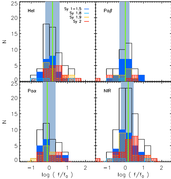
Figure 12. Histograms of the normalized virial factor f/f_0 , i.e., BH mass deviation M_{\text{BH},\sigma_x}/M(\text{line}) , for each line subsample, as labeled in each panel. Total sample in black, Sy 1–1.5 in blue, Sy 1.8 in cyan, Sy 1.9 in orange, and Sy 2 in red. The shaded area defines the IQR , which is the region enclosing the 25th to the 75th percentile of the total distribution. The 50th percentile is overplotted with a solid green vertical line.
