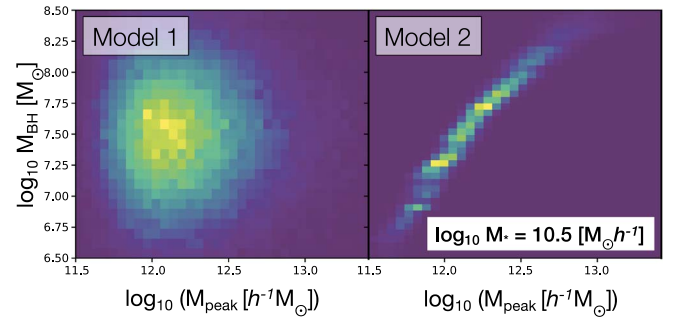
Figure 4. 2D distributions of the mock SMBH masses ( M_{\text{BH}} ) in each model example (Model 1: left; Model 2: right) at fixed stellar mass \log_{10}(M_*) = 10.5 ( M_{\odot} h^{-1} ) as a function of host peak (sub)halo mass ( M_{\text{peak}} ), demonstrating the different assumptions between M_{\text{BH}} and M_{\text{peak}} for each model.
