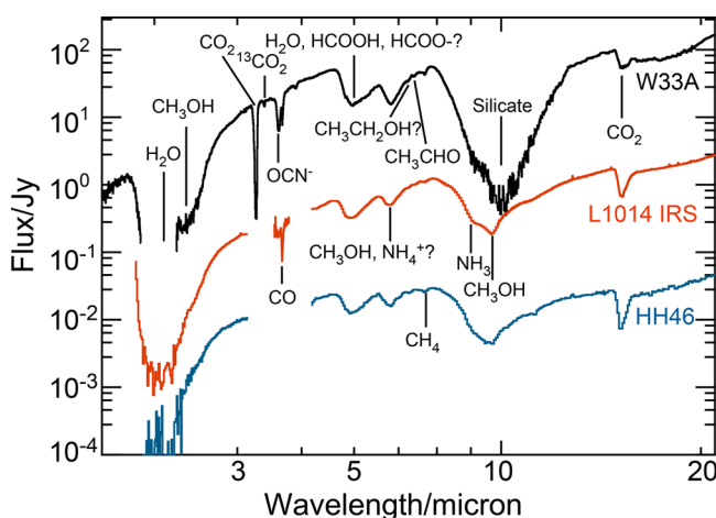
Figure 3. Spectra of interstellar ice absorptions seen toward 3 protostellar objects. Spectrum taken from Öberg et al. 16 Copyright 2011 IOP Publishing.
